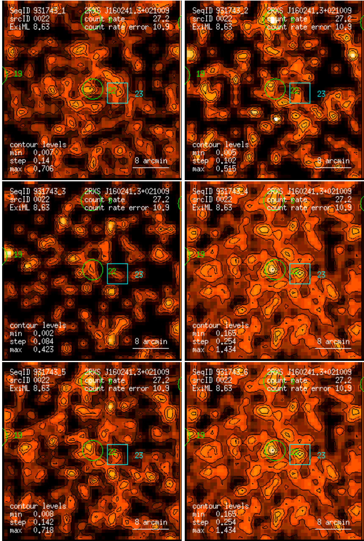
Figure 22: RASS 931743: detection 0022: band rate images, Gaussian filter: (1) PSPC channels 11 – 41, (2) 52 – 90, (3) 91 – 201, (4) 11 – 235, (5) 52 – 201, (6) 11 – 201. Broad band rates in counts/ks. Band rate contour levels in counts/ks/arcmin 2 .
