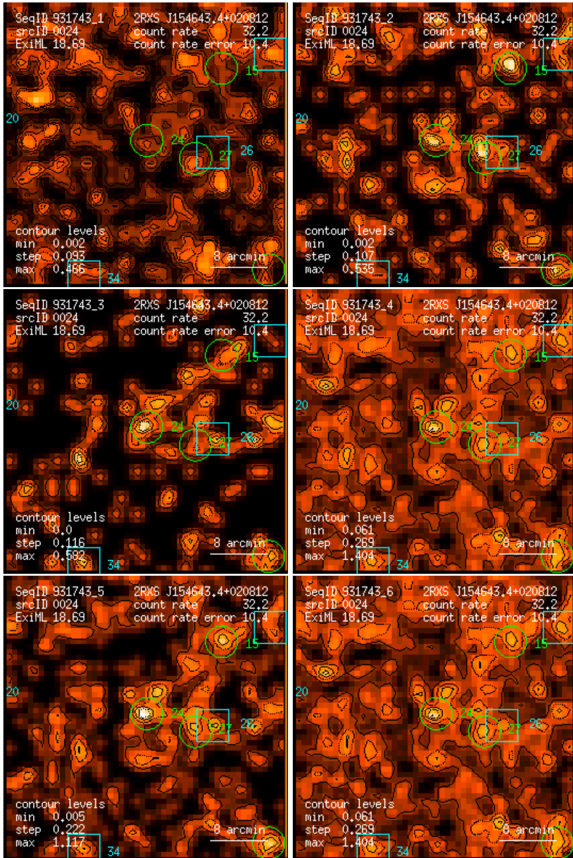
Figure 24: RASS 931743: detection 0024: band rate images, Gaussian filter: (1) PSPC channels 11 – 41, (2) 52 – 90, (3) 91 – 201, (4) 11 – 235, (5) 52 – 201, (6) 11 – 201. Broad band rates in counts/ks. Band rate contour levels in counts/ks/arcmin 2 .
