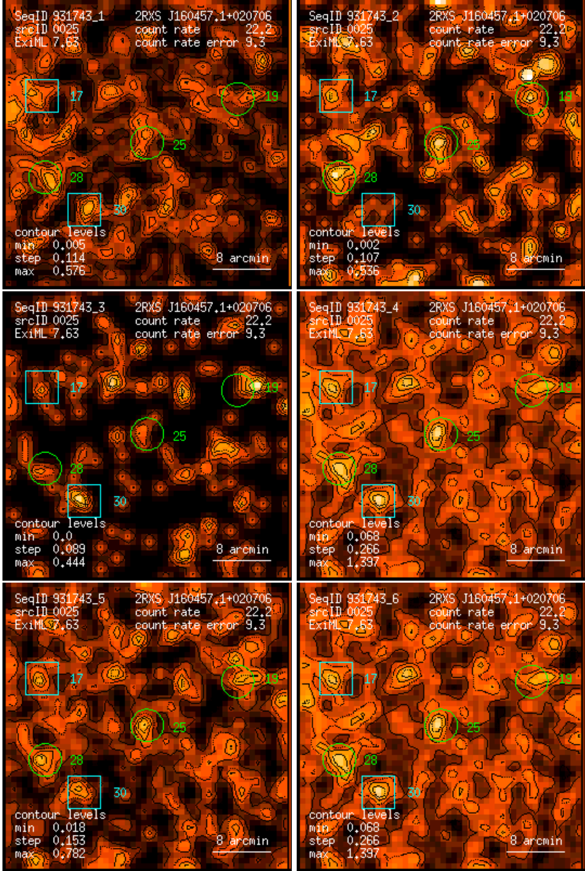
Figure 25: RASS 931743: detection 0025: band rate images, Gaussian filter: (1) PSPC channels 11 – 41, (2) 52 – 90, (3) 91 – 201, (4) 11 – 235, (5) 52 – 201, (6) 11 – 201. Broad band rates in counts/ks. Band rate contour levels in counts/ks/arcmin 2 .
