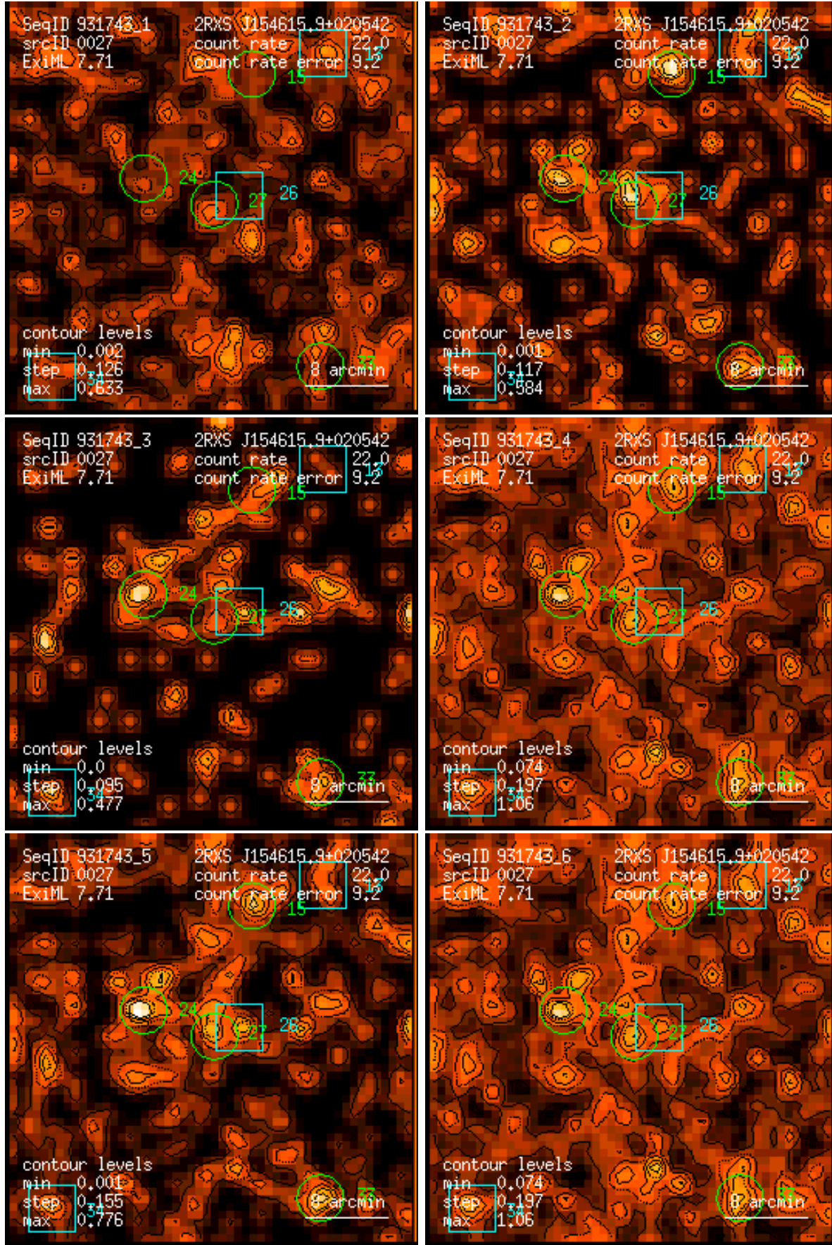
Figure 27: RASS 931743: detection 0027: band rate images, Gaussian filter: (1) PSPC channels 11 – 41, (2) 52 – 90, (3) 91 – 201, (4) 11 – 235, (5) 52 – 201, (6) 11 – 201. Broad band rates in counts/ks. Band rate contour levels in counts/ks/arcmin 2 .
