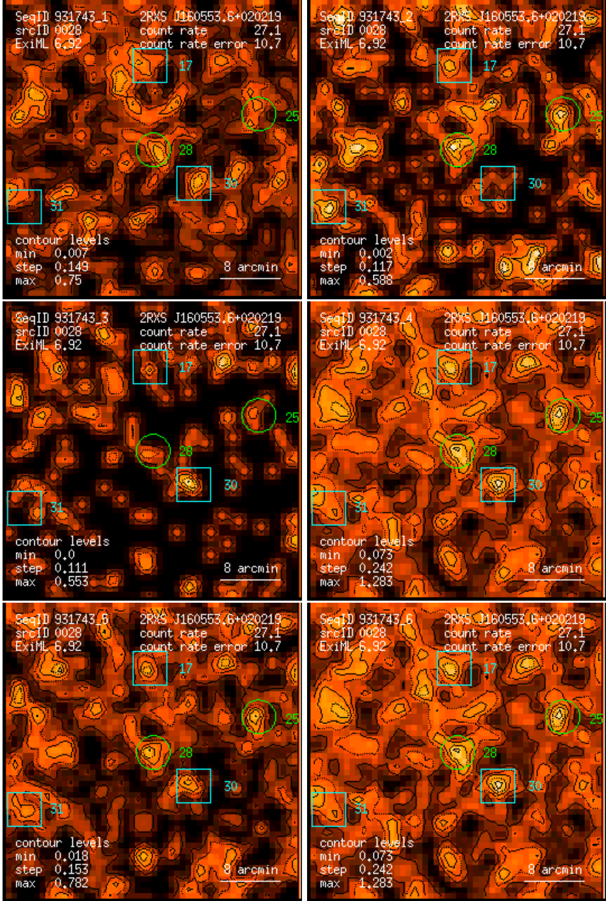
Figure 28: RASS 931743: detection 0028: band rate images, Gaussian filter: (1) PSPC channels 11 – 41, (2) 52 – 90, (3) 91 – 201, (4) 11 – 235, (5) 52 – 201, (6) 11 – 201. Broad band rates in counts/ks. Band rate contour levels in counts/ks/arcmin 2 .
