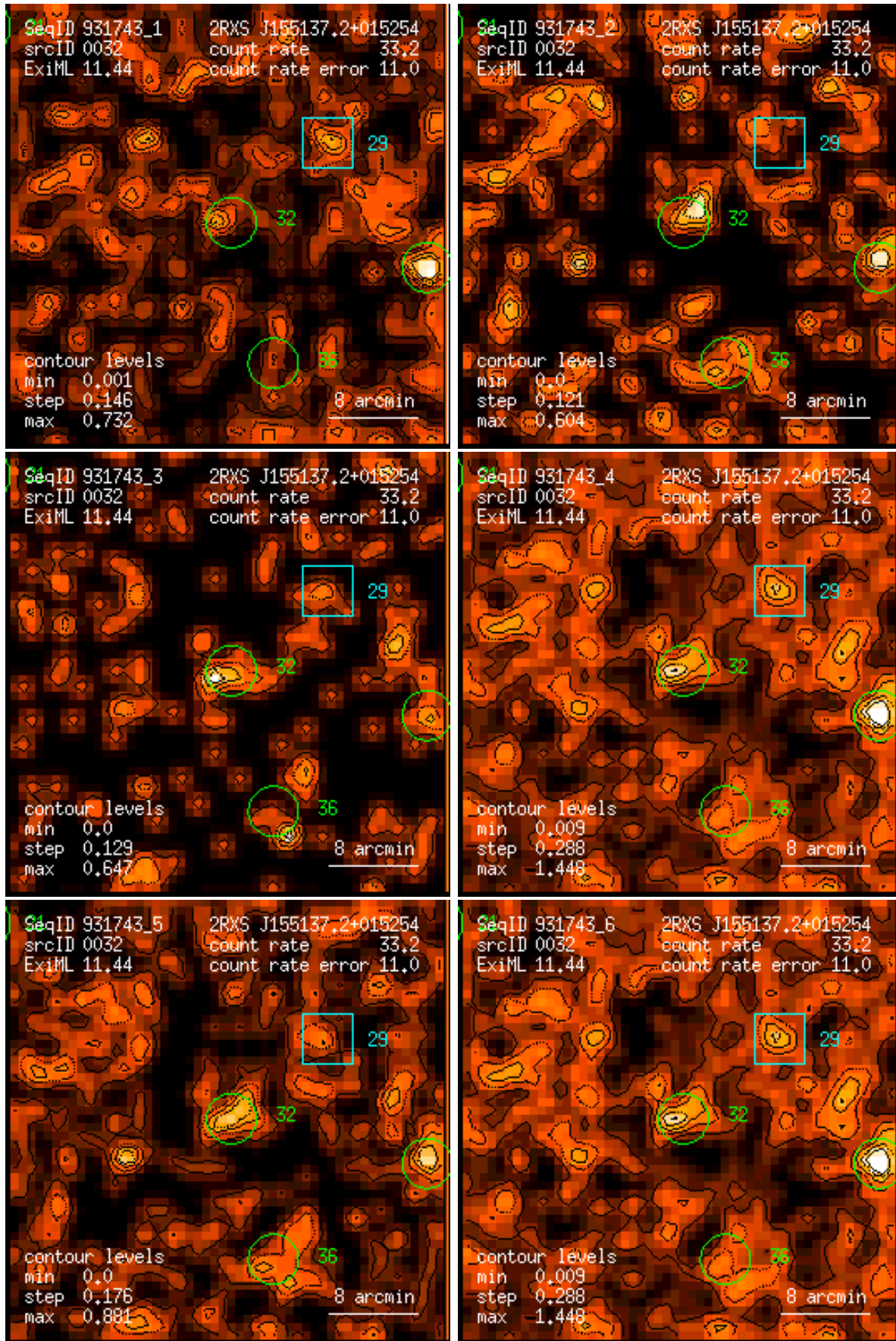
Figure 32: RASS 931743: detection 0032: band rate images, Gaussian filter: (1) PSPC channels 11 – 41, (2) 52 – 90, (3) 91 – 201, (4) 11 – 235, (5) 52 – 201, (6) 11 – 201. Broad band rates in counts/ks. Band rate contour levels in counts/ks/arcmin 2 .
