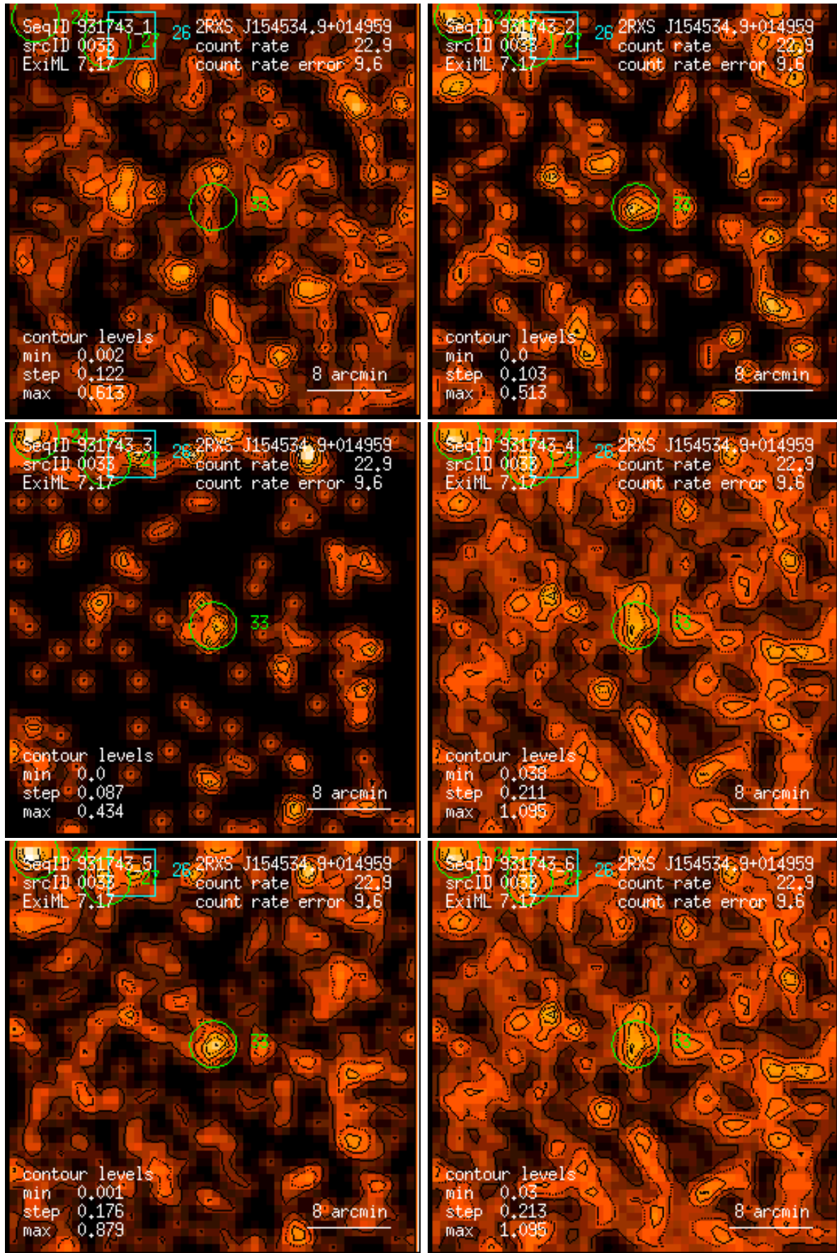
Figure 33: RASS 931743: detection 0033: band rate images, Gaussian filter: (1) PSPC channels 11 – 41, (2) 52 – 90, (3) 91 – 201, (4) 11 – 235, (5) 52 – 201, (6) 11 – 201. Broad band rates in counts/ks. Band rate contour levels in counts/ks/arcmin 2 .
