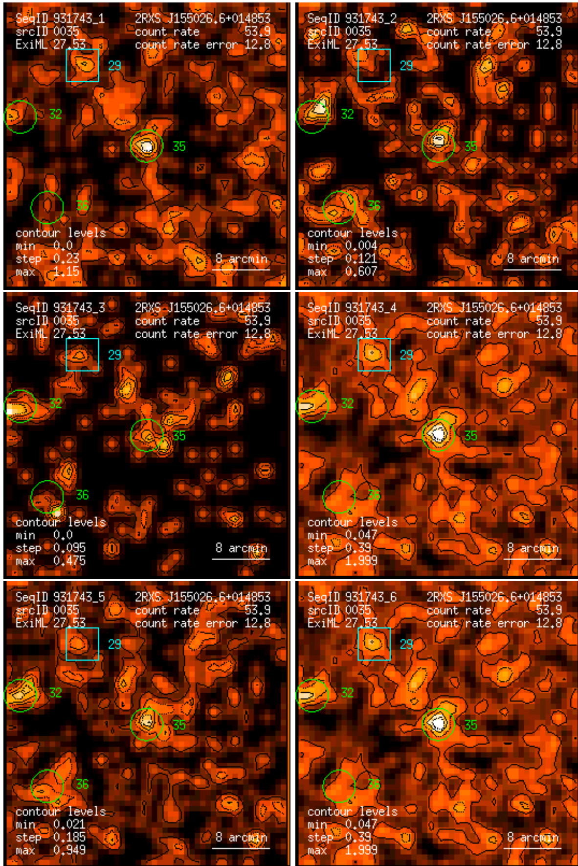
Figure 35: RASS 931743: detection 0035: band rate images, Gaussian filter: (1) PSPC channels 11 – 41, (2) 52 – 90, (3) 91 – 201, (4) 11 – 235, (5) 52 – 201, (6) 11 – 201. Broad band rates in counts/ks. Band rate contour levels in counts/ks/arcmin 2 .
