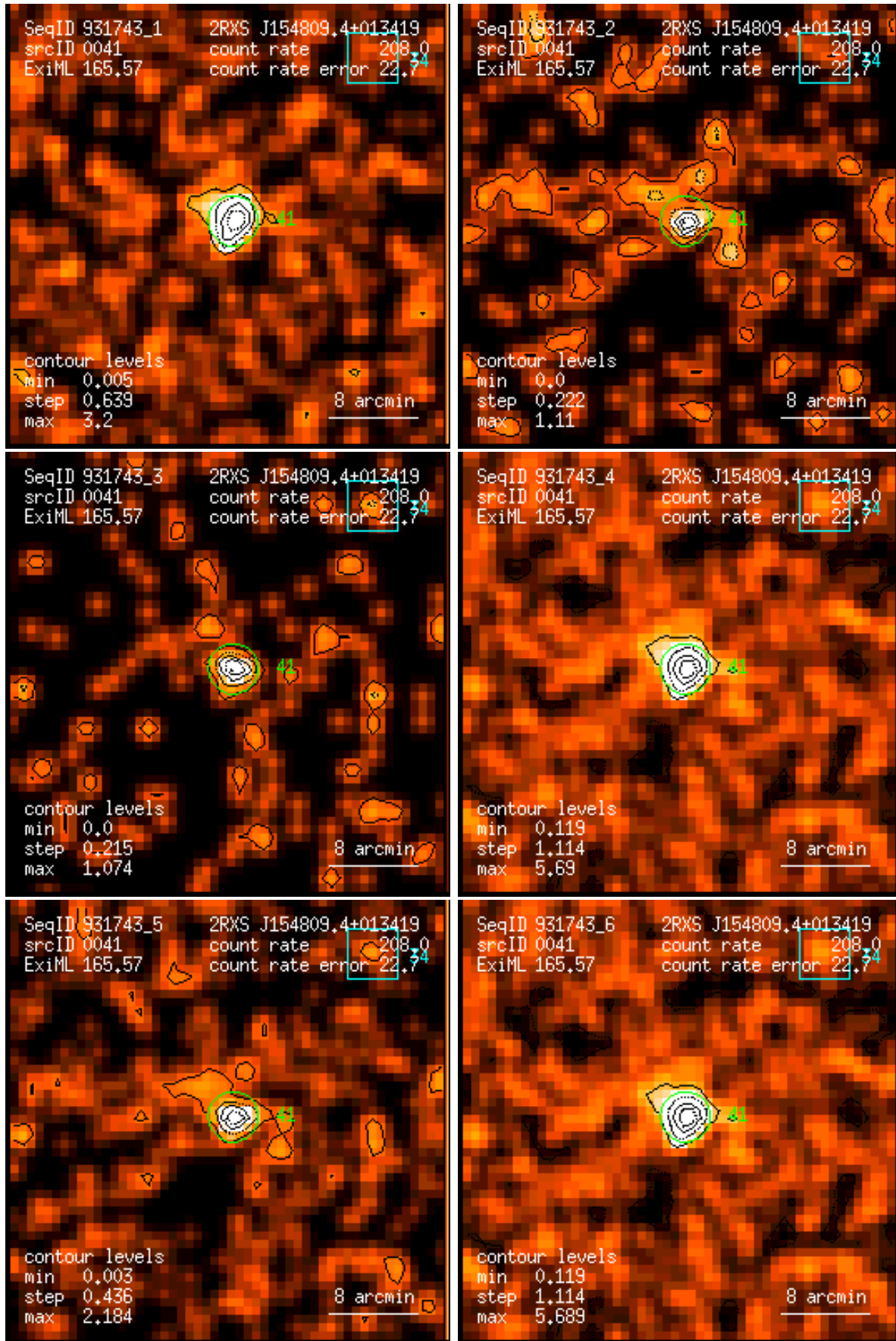
Figure 41: RASS 931743: detection 0041: band rate images, Gaussian filter: (1) PSPC channels 11 – 41, (2) 52 – 90, (3) 91 – 201, (4) 11 – 235, (5) 52 – 201, (6) 11 – 201. Broad band rates in counts/ks. Band rate contour levels in counts/ks/arcmin 2 .
