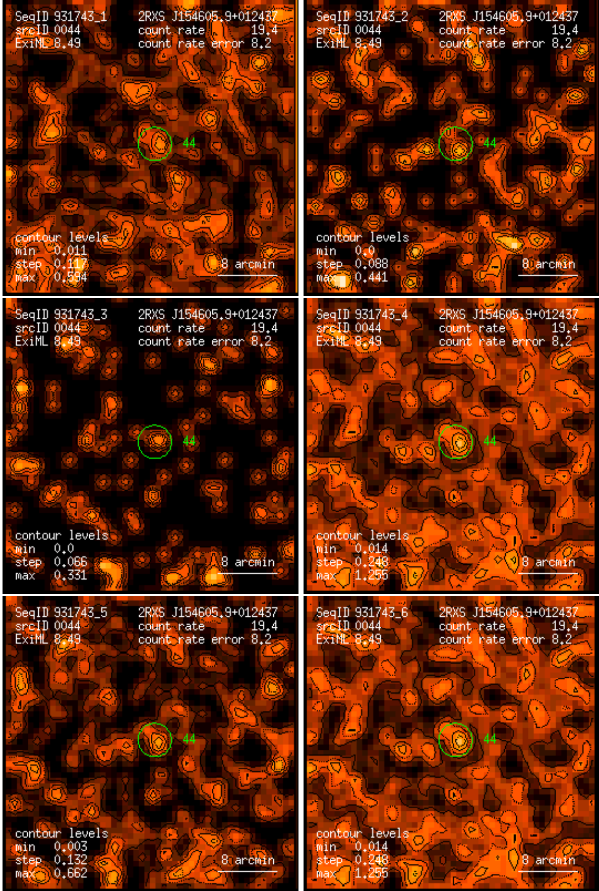
Figure 44: RASS 931743: detection 0044: band rate images, Gaussian filter: (1) PSPC channels 11 – 41, (2) 52 – 90, (3) 91 – 201, (4) 11 – 235, (5) 52 – 201, (6) 11 – 201. Broad band rates in counts/ks. Band rate contour levels in counts/ks/arcmin 2 .
