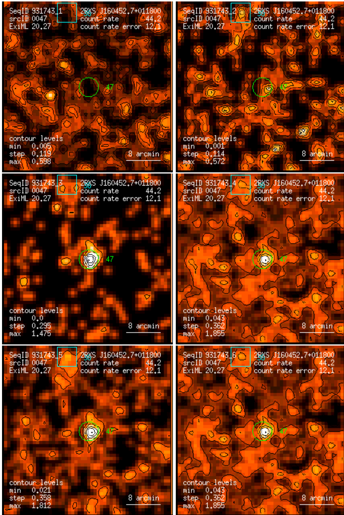
Figure 47: RASS 931743: detection 0047: band rate images, Gaussian filter: (1) PSPC channels 11 – 41, (2) 52 – 90, (3) 91 – 201, (4) 11 – 235, (5) 52 – 201, (6) 11 – 201. Broad band rates in counts/ks. Band rate contour levels in counts/ks/arcmin 2 .
