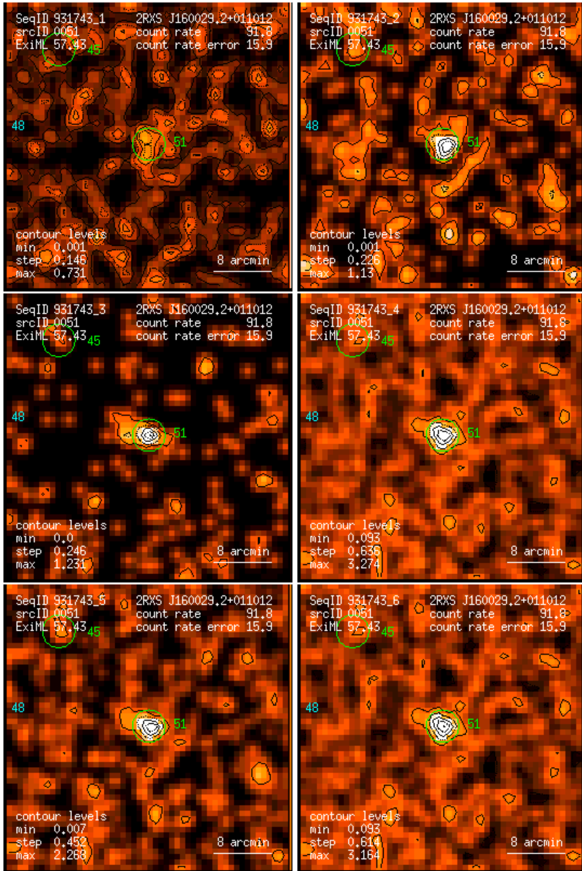
Figure 51: RASS 931743: detection 0051: band rate images, Gaussian filter: (1) PSPC channels 11 – 41, (2) 52 – 90, (3) 91 – 201, (4) 11 – 235, (5) 52 – 201, (6) 11 – 201. Broad band rates in counts/ks. Band rate contour levels in counts/ks/arcmin 2 .
