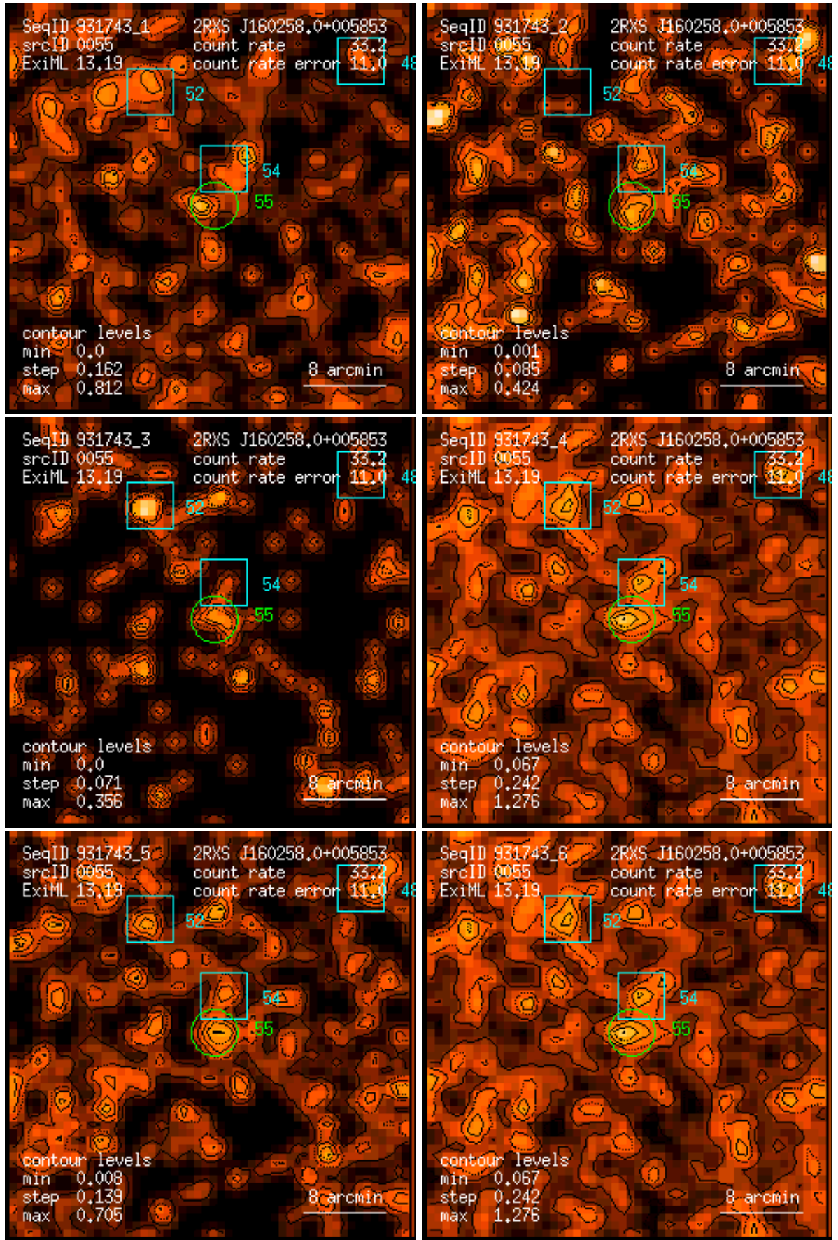
Figure 55: RASS 931743: detection 0055: band rate images, Gaussian filter: (1) PSPC channels 11 – 41, (2) 52 – 90, (3) 91 – 201, (4) 11 – 235, (5) 52 – 201, (6) 11 – 201. Broad band rates in counts/ks. Band rate contour levels in counts/ks/arcmin 2 .
