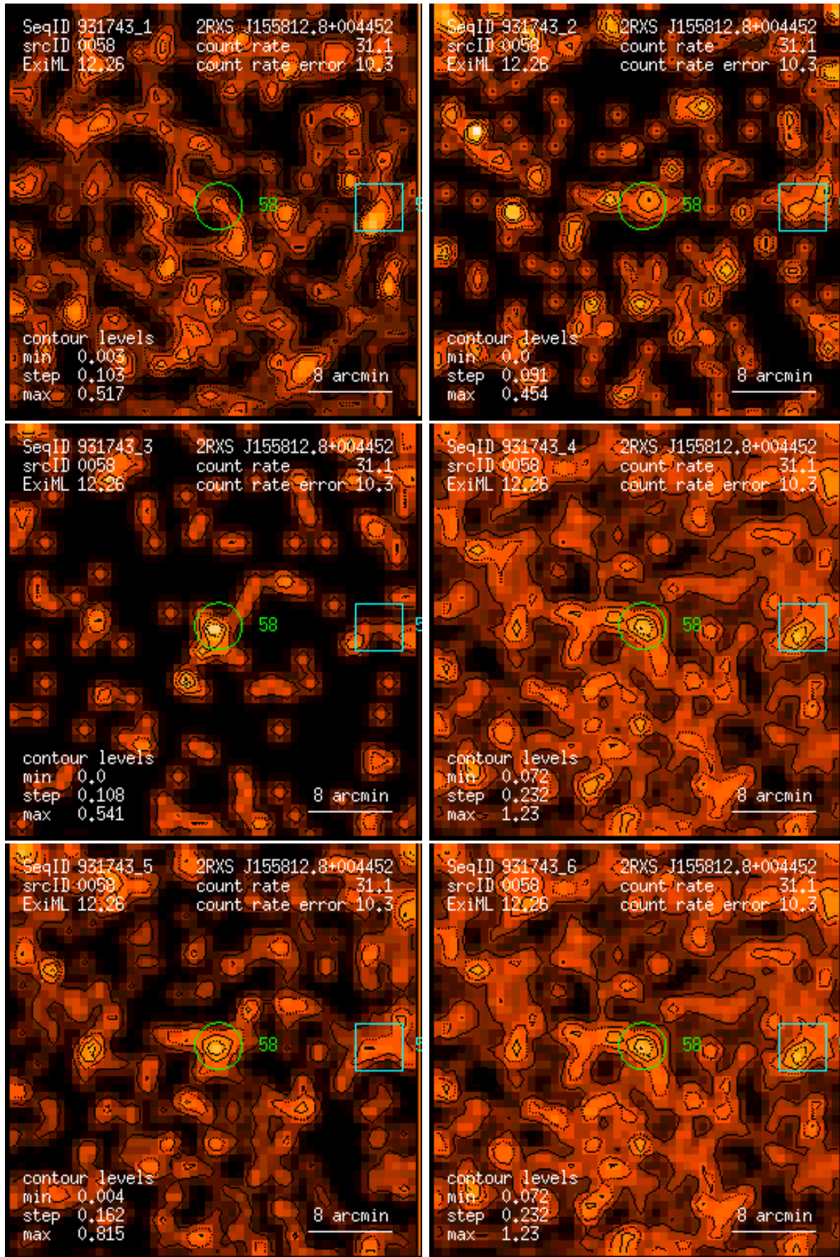
Figure 58: RASS 931743: detection 0058: band rate images, Gaussian filter: (1) PSPC channels 11 – 41, (2) 52 – 90, (3) 91 – 201, (4) 11 – 235, (5) 52 – 201, (6) 11 – 201. Broad band rates in counts/ks. Band rate contour levels in counts/ks/arcmin 2 .
