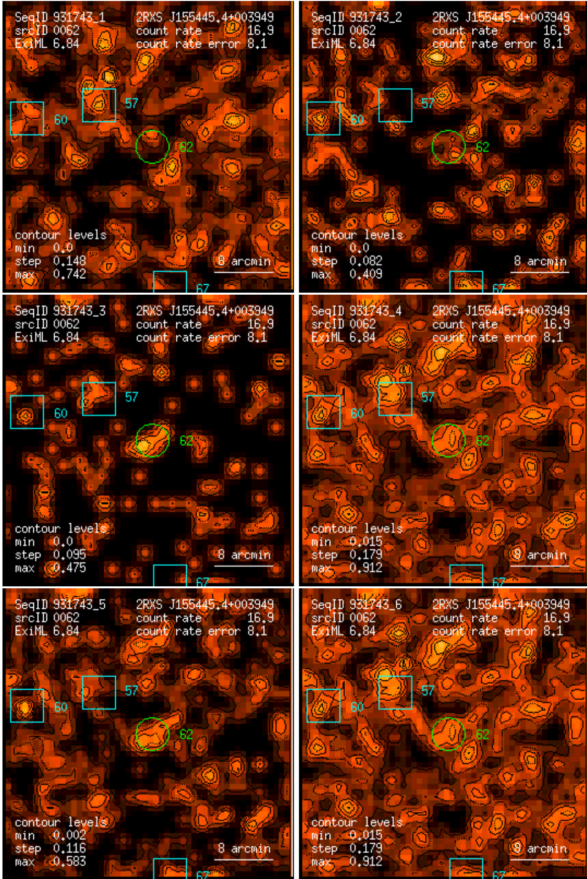
Figure 62: RASS 931743: detection 0062: band rate images, Gaussian filter: (1) PSPC channels 11 – 41, (2) 52 – 90, (3) 91 – 201, (4) 11 – 235, (5) 52 – 201, (6) 11 – 201. Broad band rates in counts/ks. Band rate contour levels in counts/ks/arcmin 2 .
