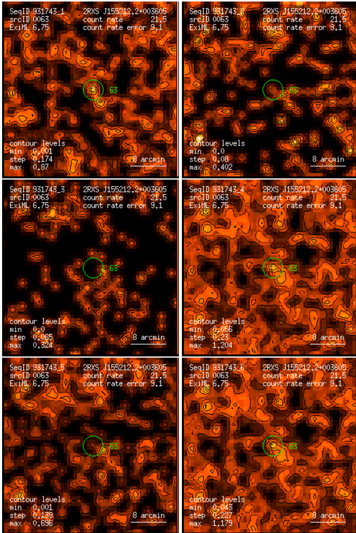
Figure 63: RASS 931743: detection 0063: band rate images, Gaussian filter: (1) PSPC channels 11 – 41, (2) 52 – 90, (3) 91 – 201, (4) 11 – 235, (5) 52 – 201, (6) 11 – 201. Broad band rates in counts/ks. Band rate contour levels in counts/ks/arcmin 2 .
