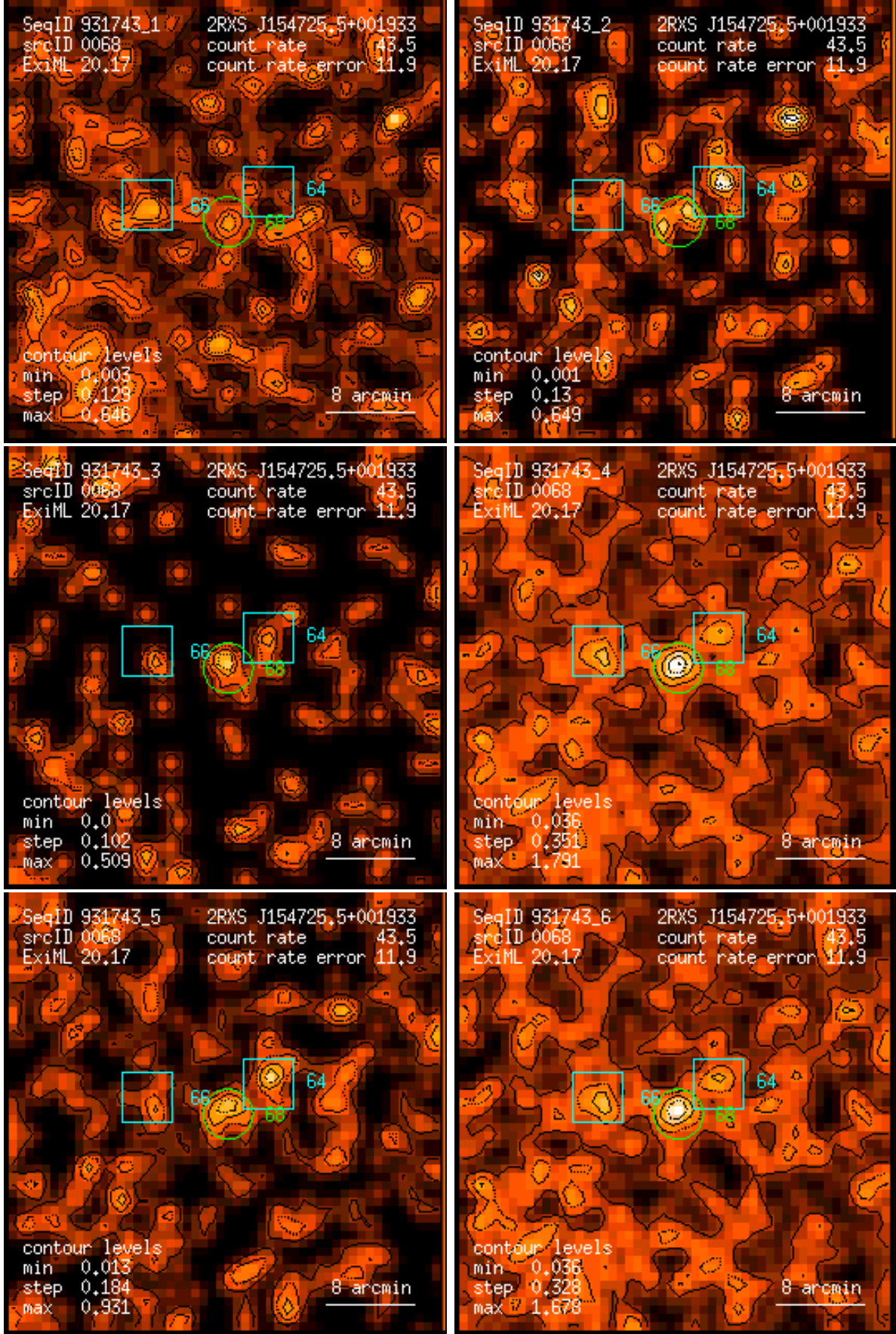
Figure 68: RASS 931743: detection 0068: band rate images, Gaussian filter: (1) PSPC channels 11 – 41, (2) 52 – 90, (3) 91 – 201, (4) 11 – 235, (5) 52 – 201, (6) 11 – 201. Broad band rates in counts/ks. Band rate contour levels in counts/ks/arcmin 2 .
