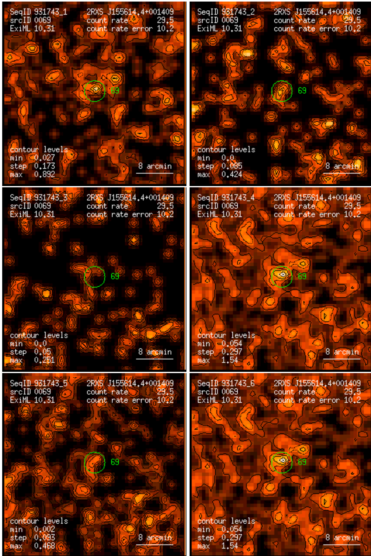
Figure 69: RASS 931743: detection 0069: band rate images, Gaussian filter: (1) PSPC channels 11 – 41, (2) 52 – 90, (3) 91 – 201, (4) 11 – 235, (5) 52 – 201, (6) 11 – 201. Broad band rates in counts/ks. Band rate contour levels in counts/ks/arcmin 2 .
