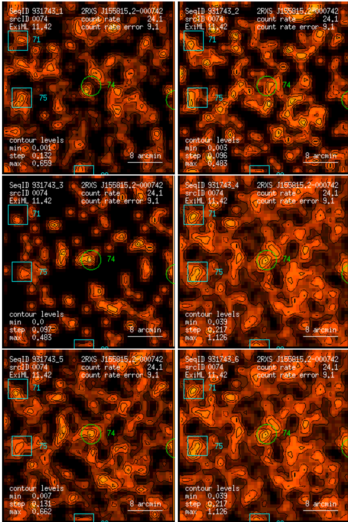
Figure 74: RASS 931743: detection 0074: band rate images, Gaussian filter: (1) PSPC channels 11 – 41, (2) 52 – 90, (3) 91 – 201, (4) 11 – 235, (5) 52 – 201, (6) 11 – 201. Broad band rates in counts/ks. Band rate contour levels in counts/ks/arcmin 2 .
