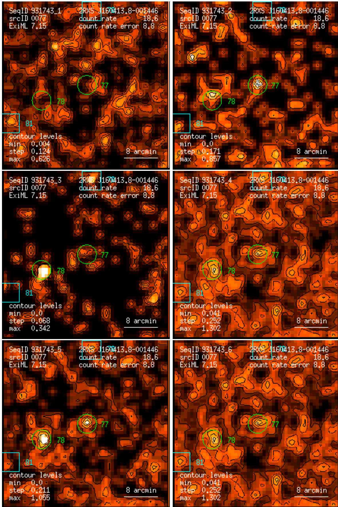
Figure 77: RASS 931743: detection 0077: band rate images, Gaussian filter: (1) PSPC channels 11 – 41, (2) 52 – 90, (3) 91 – 201, (4) 11 – 235, (5) 52 – 201, (6) 11 – 201. Broad band rates in counts/ks. Band rate contour levels in counts/ks/arcmin 2 .
