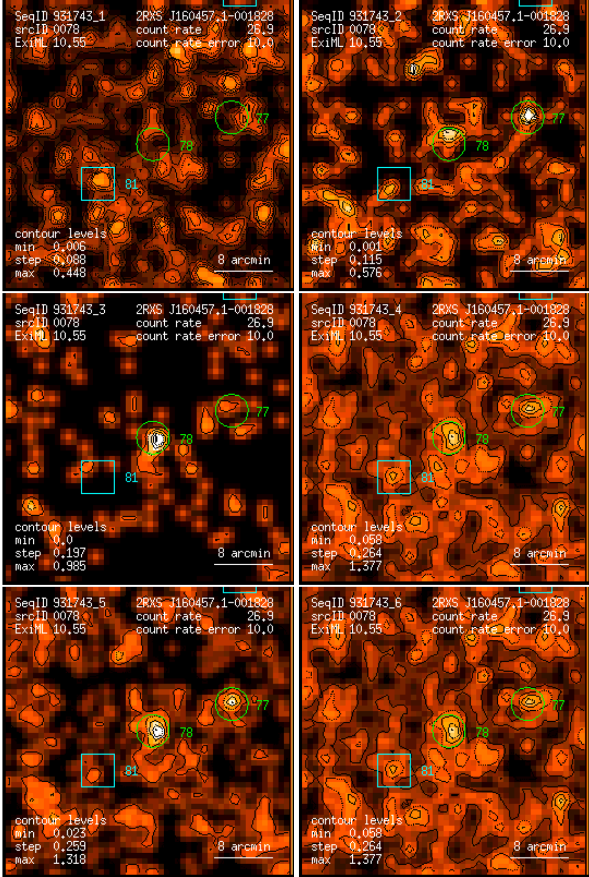
Figure 78: RASS 931743: detection 0078: band rate images, Gaussian filter: (1) PSPC channels 11 – 41, (2) 52 – 90, (3) 91 – 201, (4) 11 – 235, (5) 52 – 201, (6) 11 – 201. Broad band rates in counts/ks. Band rate contour levels in counts/ks/arcmin 2 .
