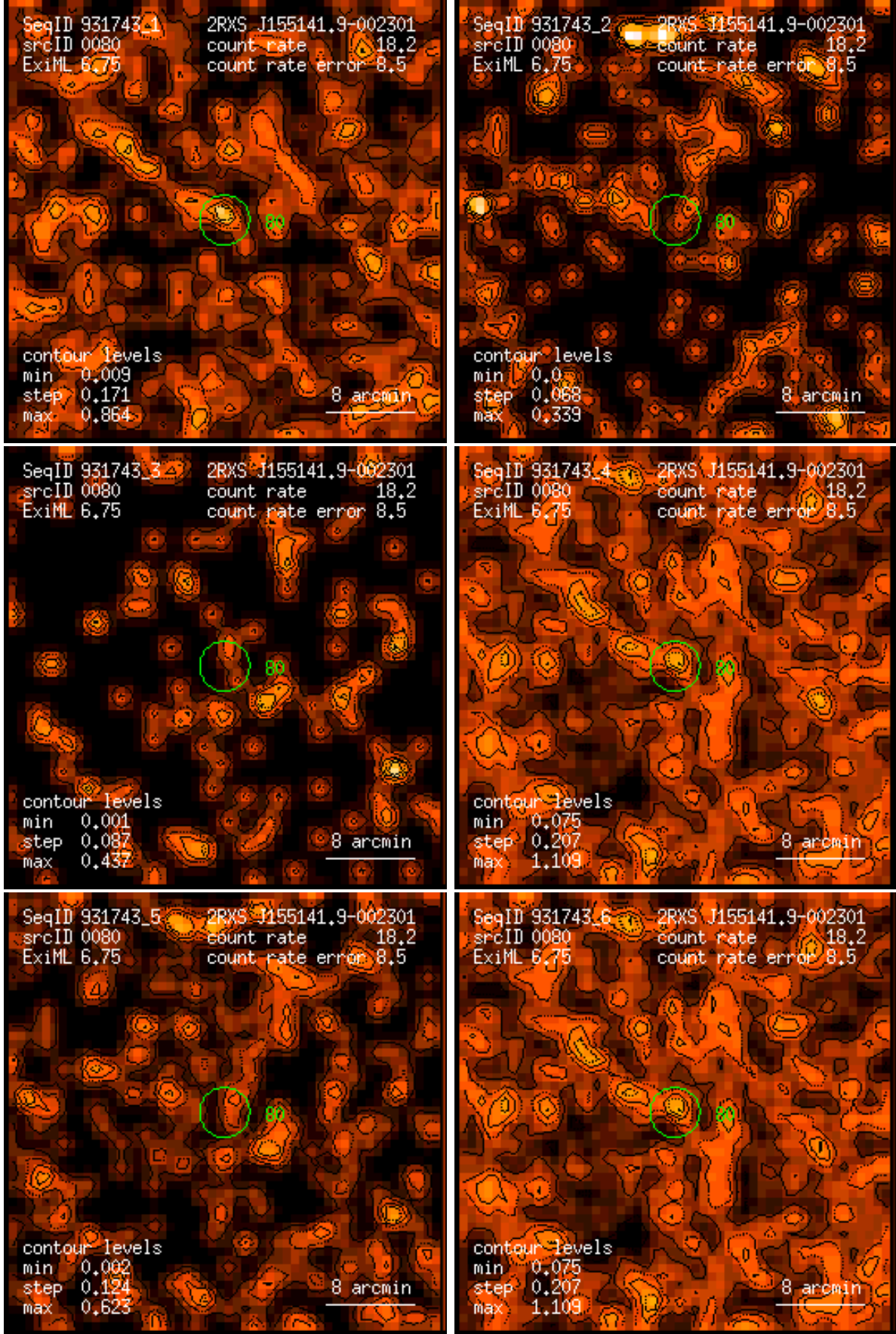
Figure 80: RASS 931743: detection 0080: band rate images, Gaussian filter: (1) PSPC channels 11 – 41, (2) 52 – 90, (3) 91 – 201, (4) 11 – 235, (5) 52 – 201, (6) 11 – 201. Broad band rates in counts/ks. Band rate contour levels in counts/ks/arcmin 2 .
