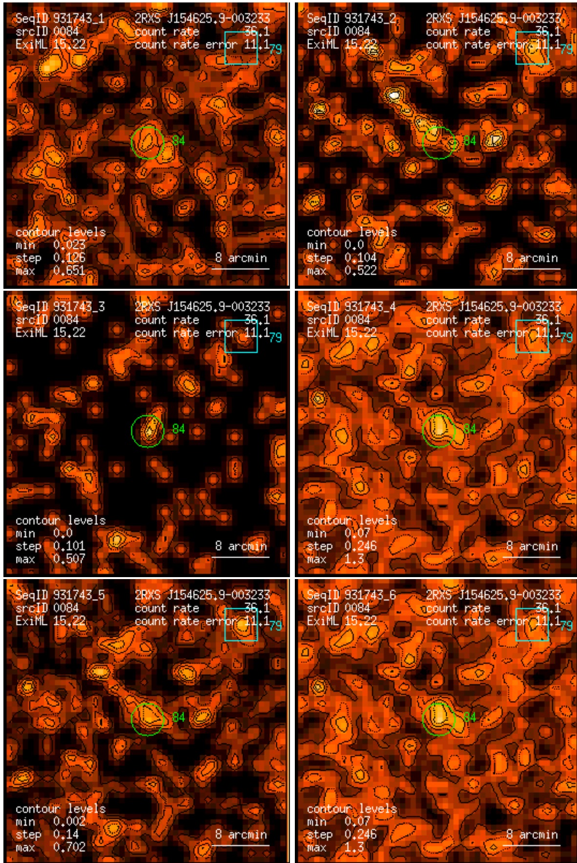
Figure 84: RASS 931743: detection 0084: band rate images, Gaussian filter: (1) PSPC channels 11 – 41, (2) 52 – 90, (3) 91 – 201, (4) 11 – 235, (5) 52 – 201, (6) 11 – 201. Broad band rates in counts/ks. Band rate contour levels in counts/ks/arcmin 2 .
