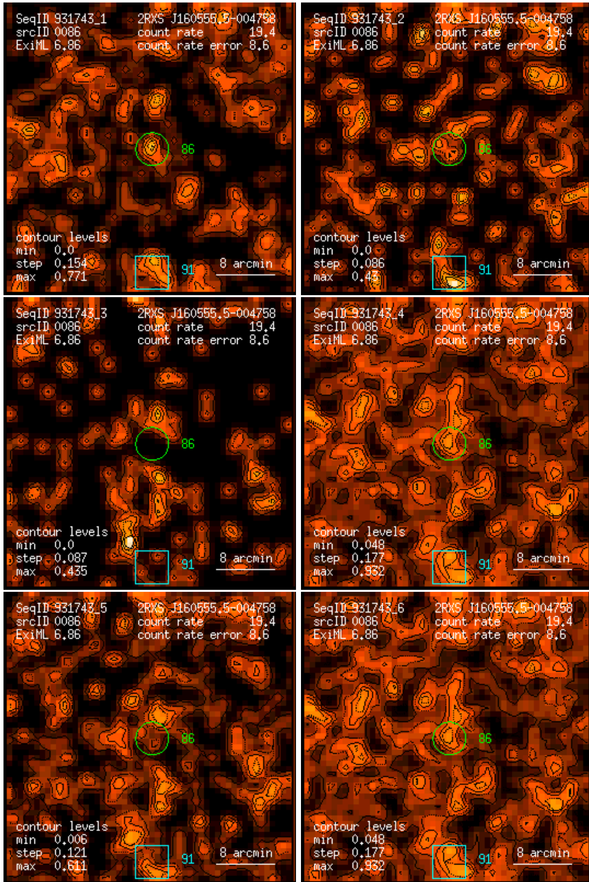
Figure 86: RASS 931743: detection 0086: band rate images, Gaussian filter: (1) PSPC channels 11 – 41, (2) 52 – 90, (3) 91 – 201, (4) 11 – 235, (5) 52 – 201, (6) 11 – 201. Broad band rates in counts/ks. Band rate contour levels in counts/ks/arcmin 2 .
