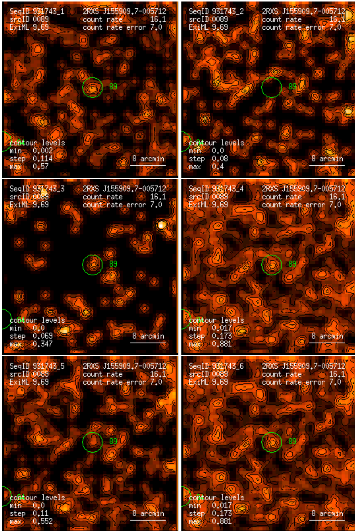
Figure 89: RASS 931743: detection 0089: band rate images, Gaussian filter: (1) PSPC channels 11 – 41, (2) 52 – 90, (3) 91 – 201, (4) 11 – 235, (5) 52 – 201, (6) 11 – 201. Broad band rates in counts/ks. Band rate contour levels in counts/ks/arcmin 2 .
