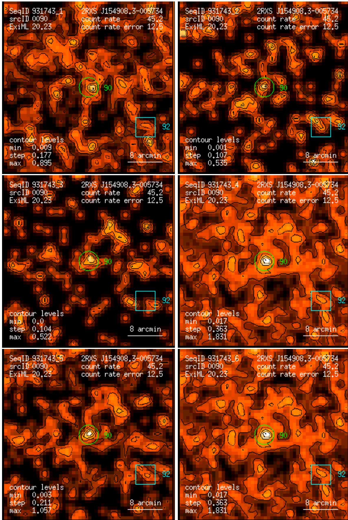
Figure 90: RASS 931743: detection 0090: band rate images, Gaussian filter: (1) PSPC channels 11 – 41, (2) 52 – 90, (3) 91 – 201, (4) 11 – 235, (5) 52 – 201, (6) 11 – 201. Broad band rates in counts/ks. Band rate contour levels in counts/ks/arcmin 2 .
