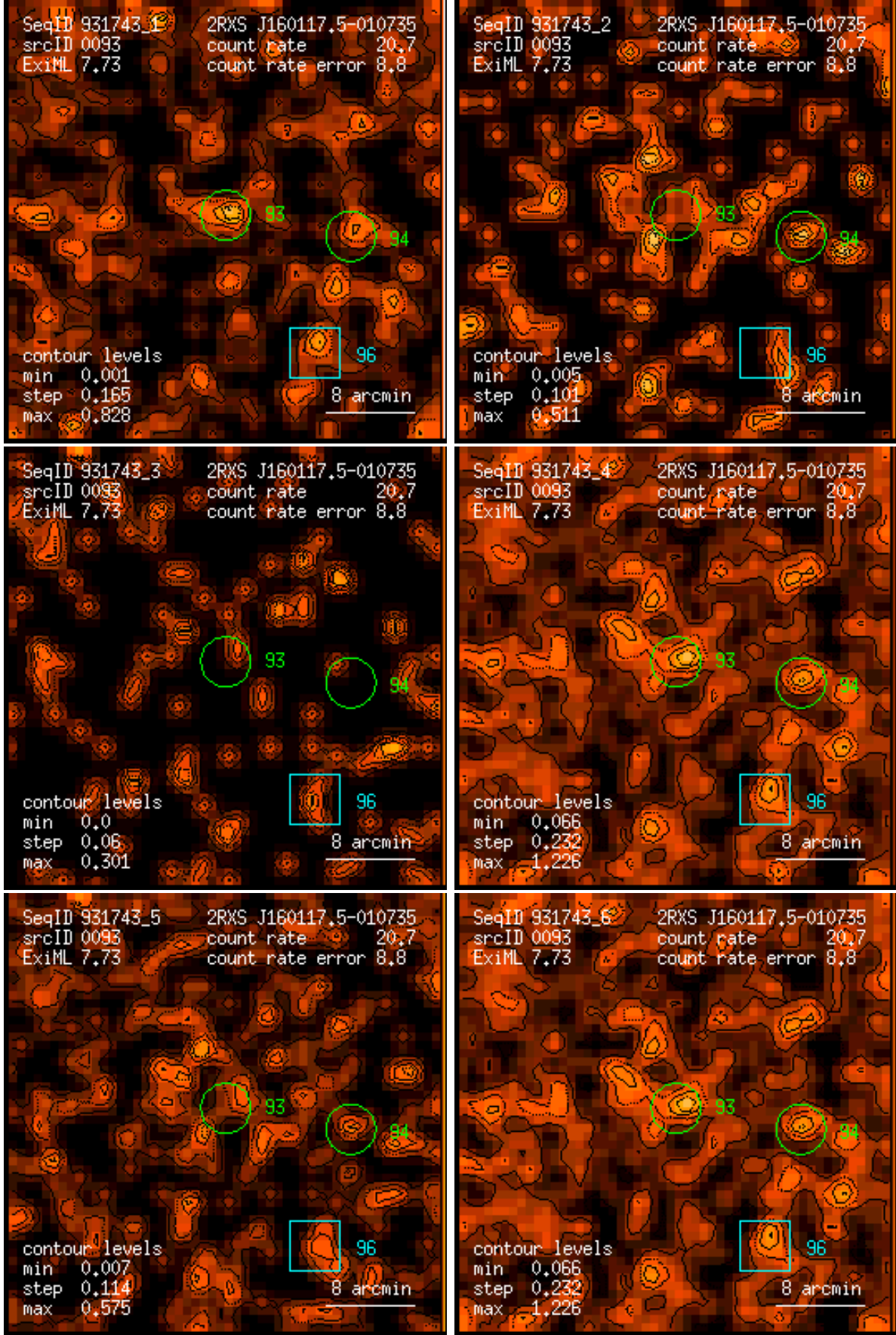
Figure 93: RASS 931743: detection 0093: band rate images, Gaussian filter: (1) PSPC channels 11 – 41, (2) 52 – 90, (3) 91 – 201, (4) 11 – 235, (5) 52 – 201, (6) 11 – 201. Broad band rates in counts/ks. Band rate contour levels in counts/ks/arcmin 2 .
