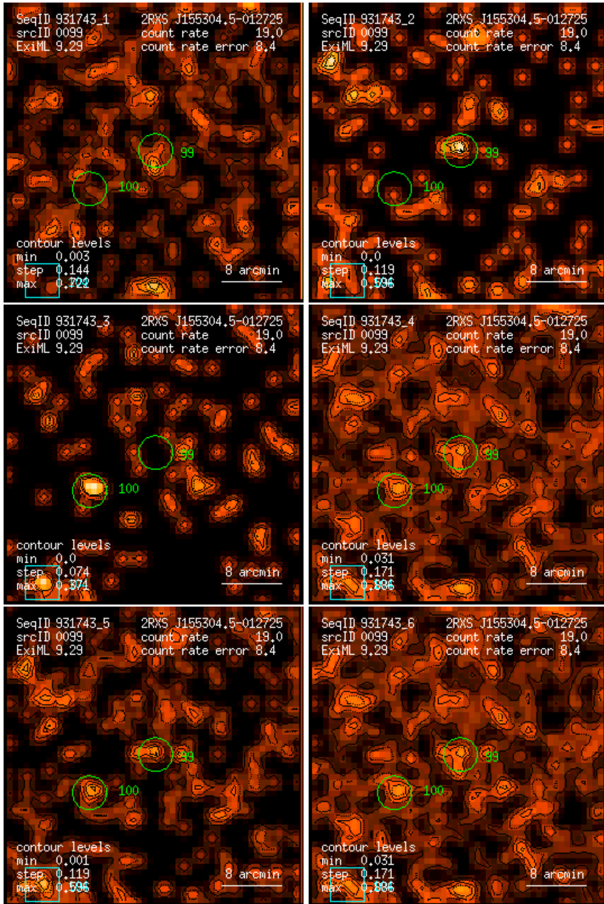
Figure 99: RASS 931743: detection 0099: band rate images, Gaussian filter: (1) PSPC channels 11 – 41, (2) 52 – 90, (3) 91 – 201, (4) 11 – 235, (5) 52 – 201, (6) 11 – 201. Broad band rates in counts/ks. Band rate contour levels in counts/ks/arcmin 2 .
