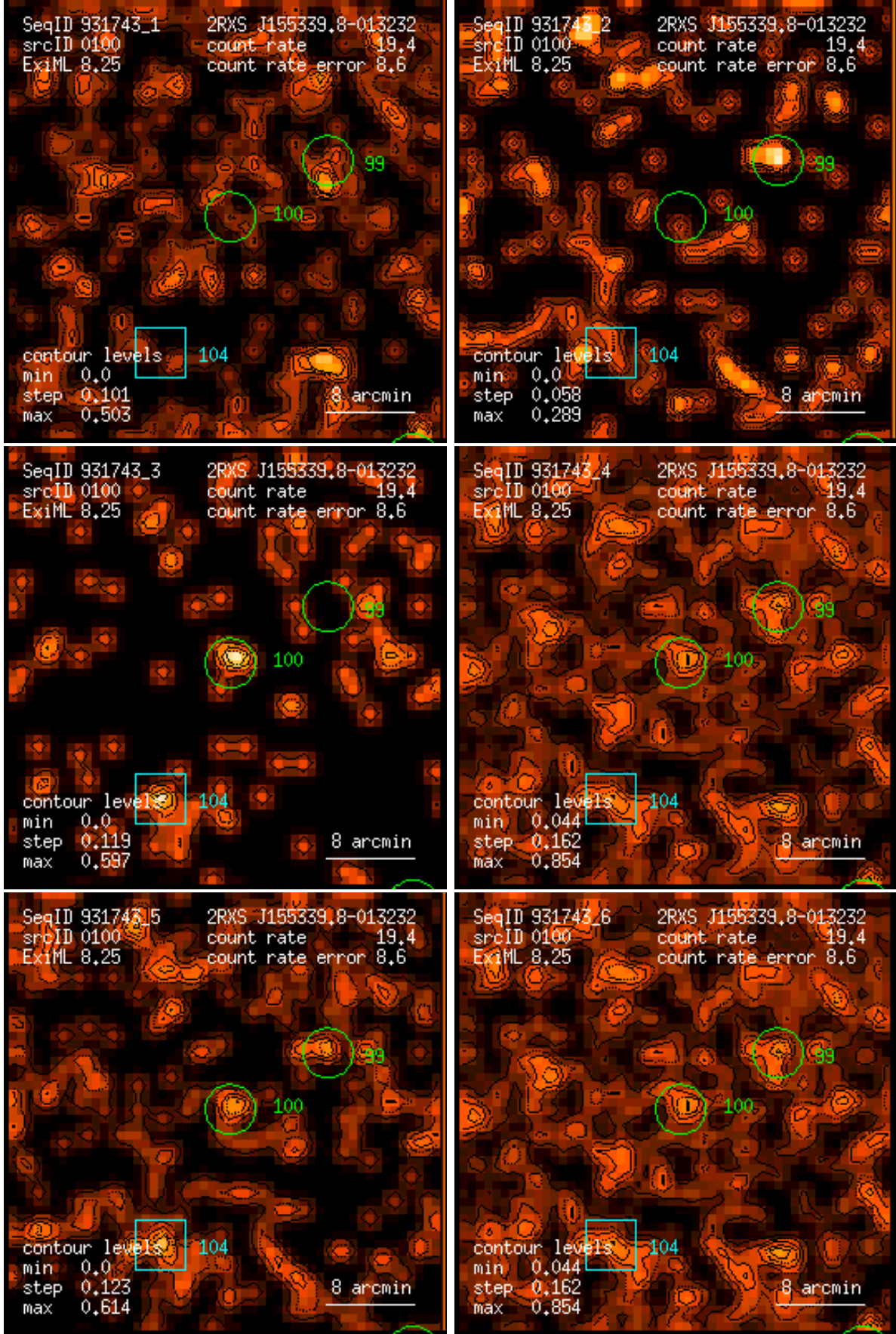
Figure 100: RASS 931743: detection 0100: band rate images, Gaussian filter: (1) PSPC channels 11 – 41, (2) 52 – 90, (3) 91 – 201, (4) 11 – 235, (5) 52 – 201, (6) 11 – 201. Broad band rates in counts/ks. Band rate contour levels in counts/ks/arcmin 2 .
