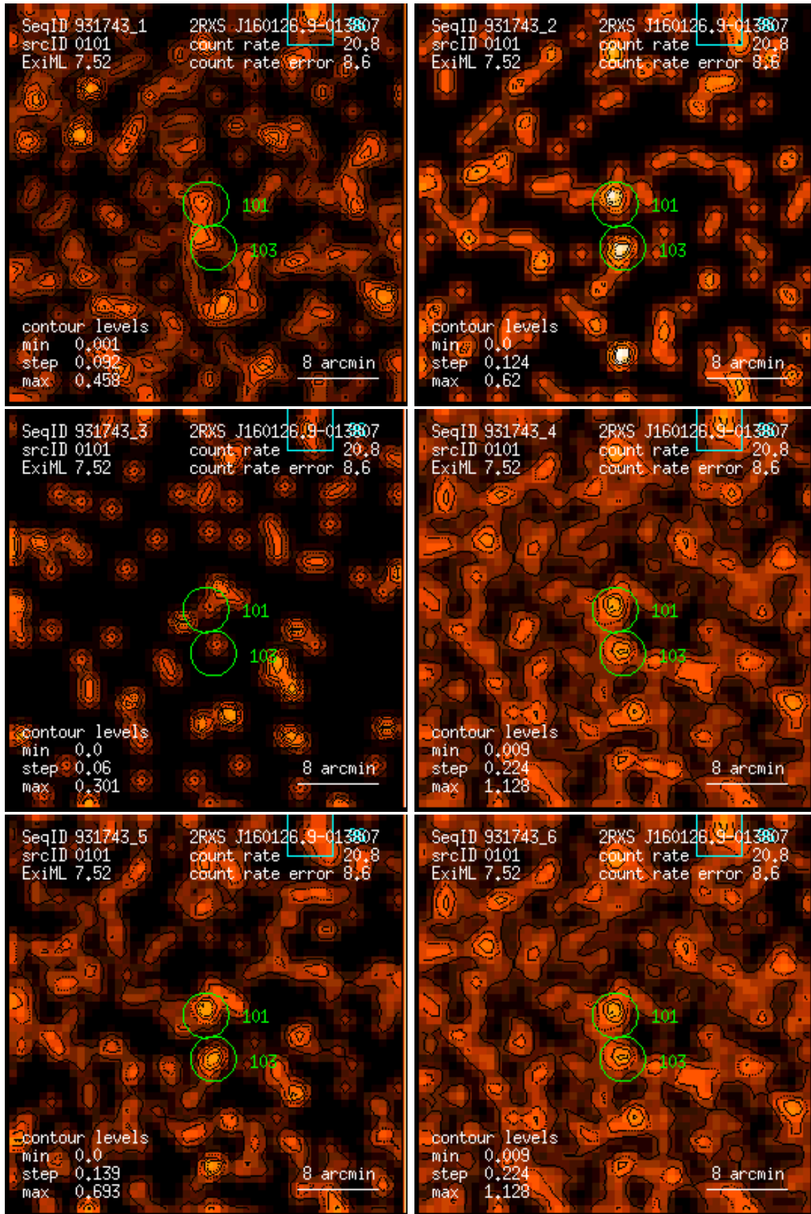
Figure 101: RASS 931743: detection 0101: band rate images, Gaussian filter: (1) PSPC channels 11 – 41, (2) 52 – 90, (3) 91 – 201, (4) 11 – 235, (5) 52 – 201, (6) 11 – 201. Broad band rates in counts/ks. Band rate contour levels in counts/ks/arcmin 2 .
