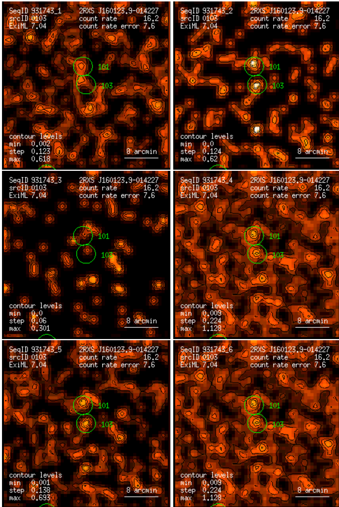
Figure 103: RASS 931743: detection 0103: band rate images, Gaussian filter: (1) PSPC channels 11 – 41, (2) 52 – 90, (3) 91 – 201, (4) 11 – 235, (5) 52 – 201, (6) 11 – 201. Broad band rates in counts/ks. Band rate contour levels in counts/ks/arcmin 2 .
