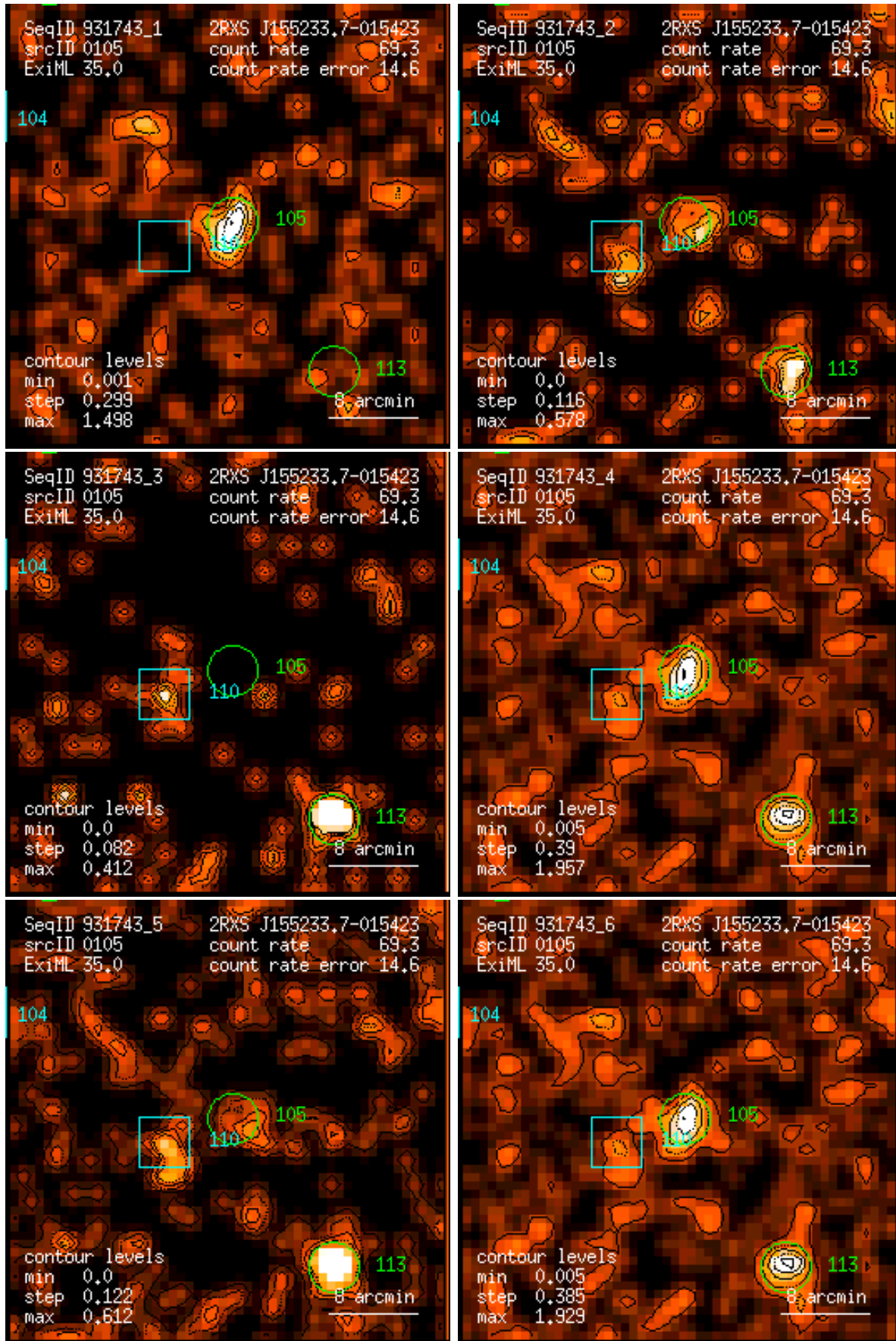
Figure 105: RASS 931743: detection 0105: band rate images, Gaussian filter: (1) PSPC channels 11 – 41, (2) 52 – 90, (3) 91 – 201, (4) 11 – 235, (5) 52 – 201, (6) 11 – 201. Broad band rates in counts/ks. Band rate contour levels in counts/ks/arcmin 2 .
