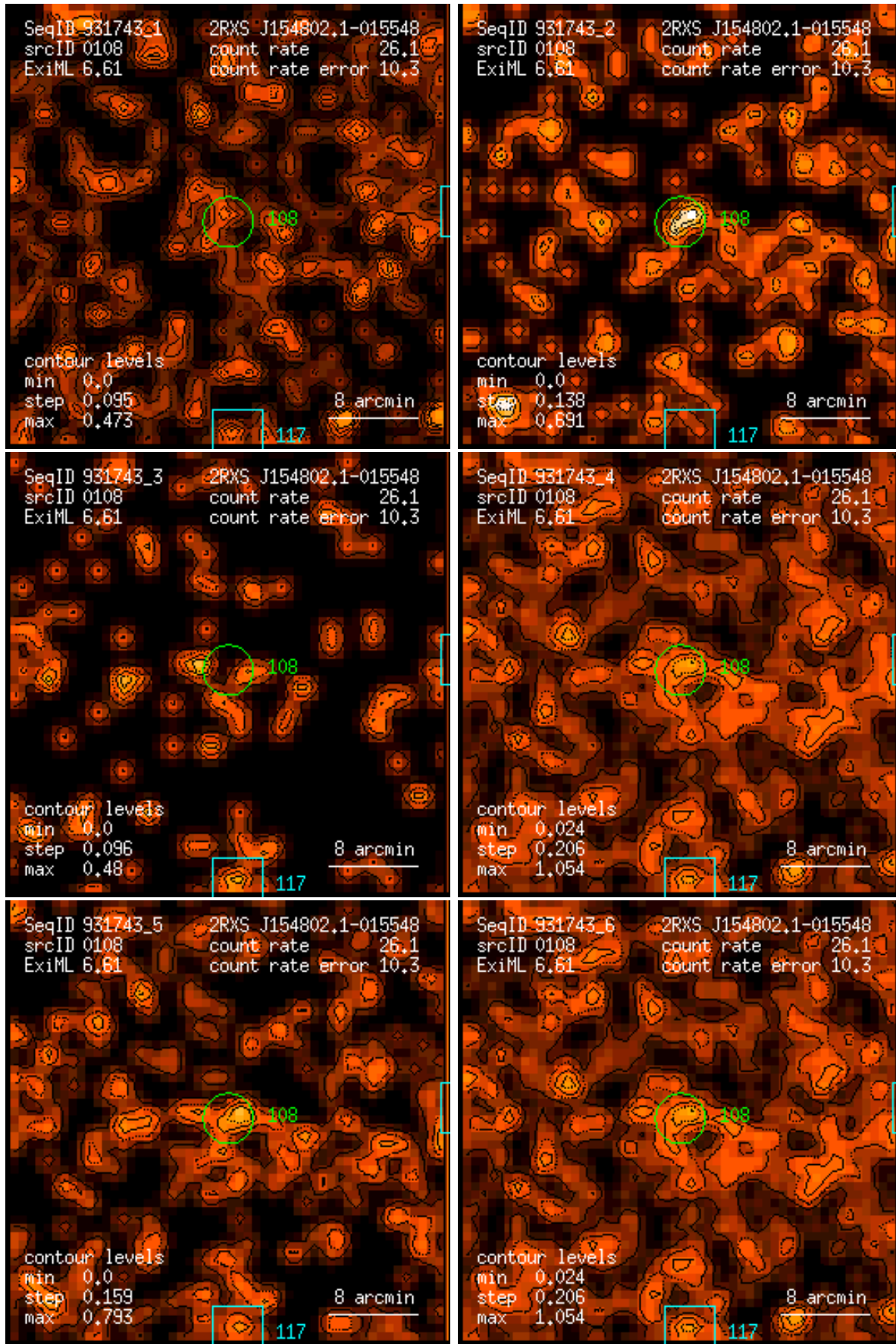
Figure 108: RASS 931743: detection 0108: band rate images, Gaussian filter: (1) PSPC channels 11 – 41, (2) 52 – 90, (3) 91 – 201, (4) 11 – 235, (5) 52 – 201, (6) 11 – 201. Broad band rates in counts/ks. Band rate contour levels in counts/ks/arcmin 2 .
