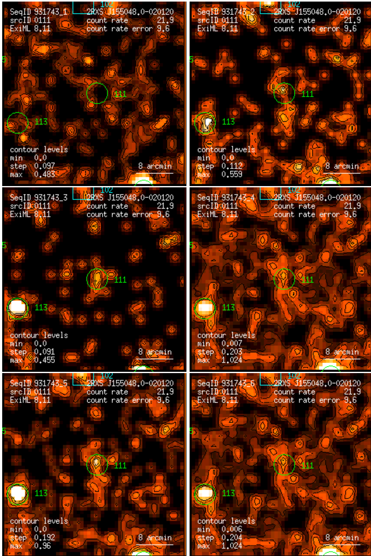
Figure 111: RASS 931743: detection 0111: band rate images, Gaussian filter: (1) PSPC channels 11 – 41, (2) 52 – 90, (3) 91 – 201, (4) 11 – 235, (5) 52 – 201, (6) 11 – 201. Broad band rates in counts/ks. Band rate contour levels in counts/ks/arcmin 2 .
