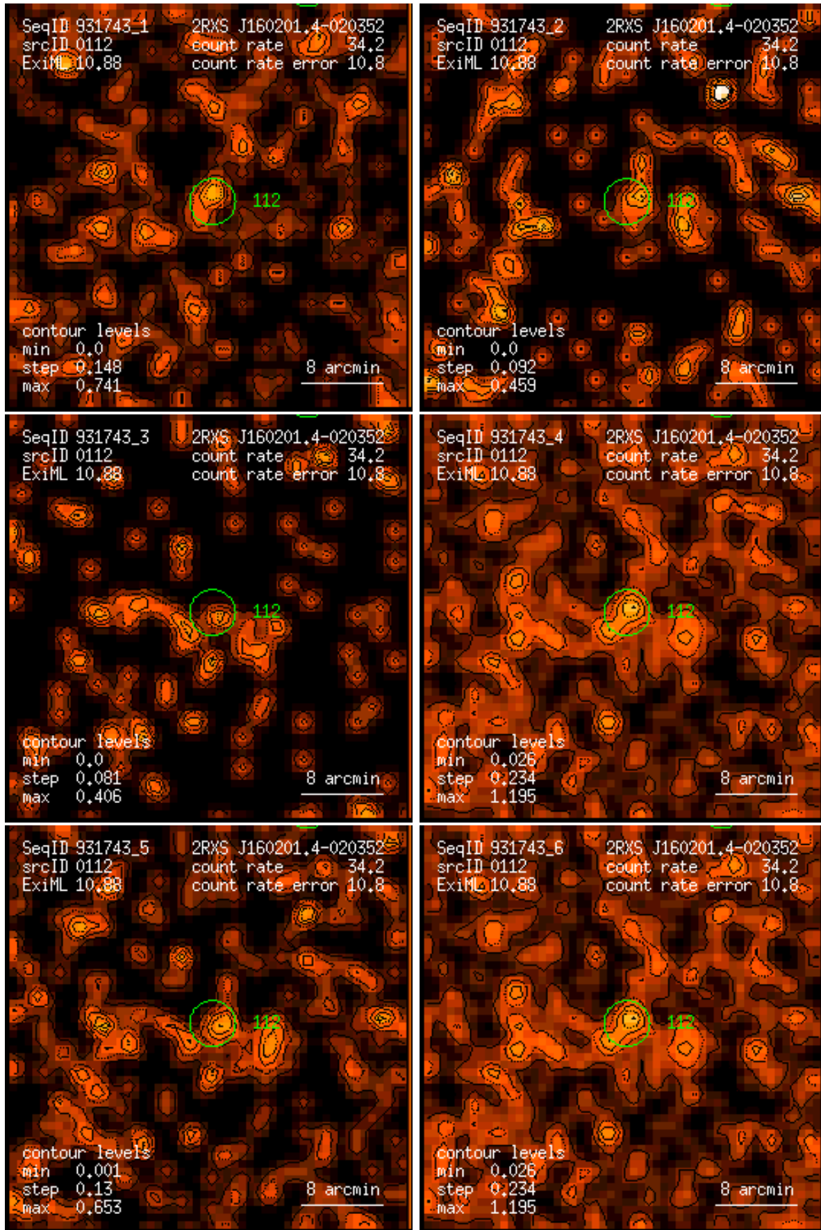
Figure 112: RASS 931743: detection 0112: band rate images, Gaussian filter: (1) PSPC channels 11 – 41, (2) 52 – 90, (3) 91 – 201, (4) 11 – 235, (5) 52 – 201, (6) 11 – 201. Broad band rates in counts/ks. Band rate contour levels in counts/ks/arcmin 2 .
