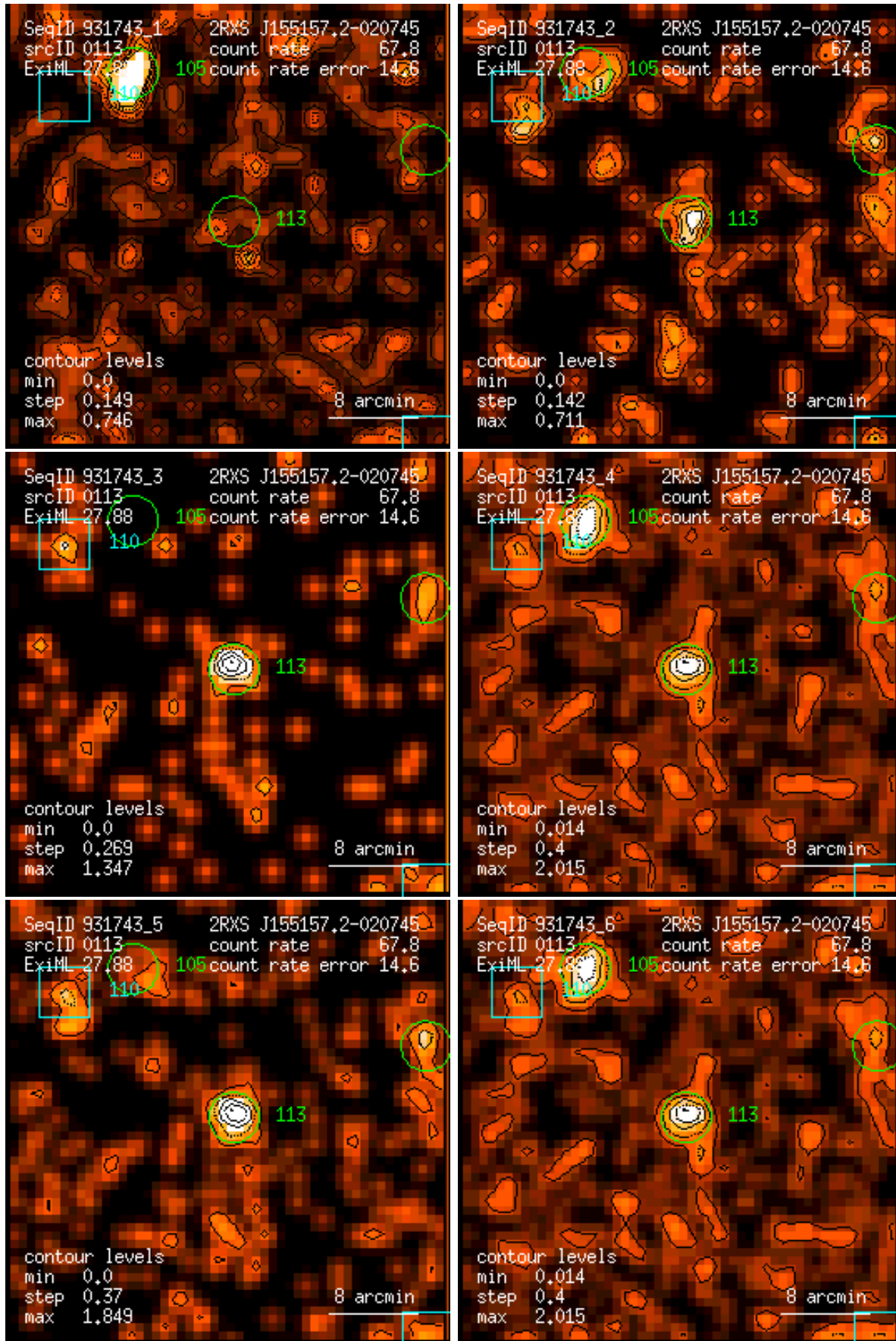
Figure 113: RASS 931743: detection 0113: band rate images, Gaussian filter: (1) PSPC channels 11 – 41, (2) 52 – 90, (3) 91 – 201, (4) 11 – 235, (5) 52 – 201, (6) 11 – 201. Broad band rates in counts/ks. Band rate contour levels in counts/ks/arcmin 2 .
