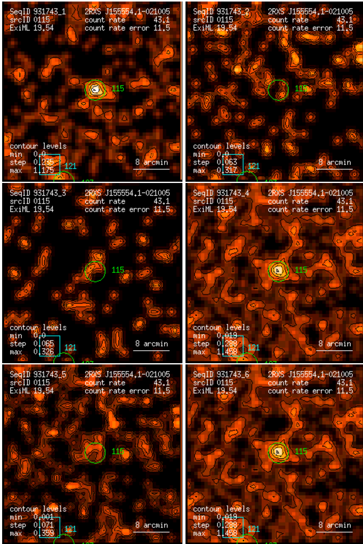
Figure 115: RASS 931743: detection 0115: band rate images, Gaussian filter: (1) PSPC channels 11 – 41, (2) 52 – 90, (3) 91 – 201, (4) 11 – 235, (5) 52 – 201, (6) 11 – 201. Broad band rates in counts/ks. Band rate contour levels in counts/ks/arcmin 2 .
