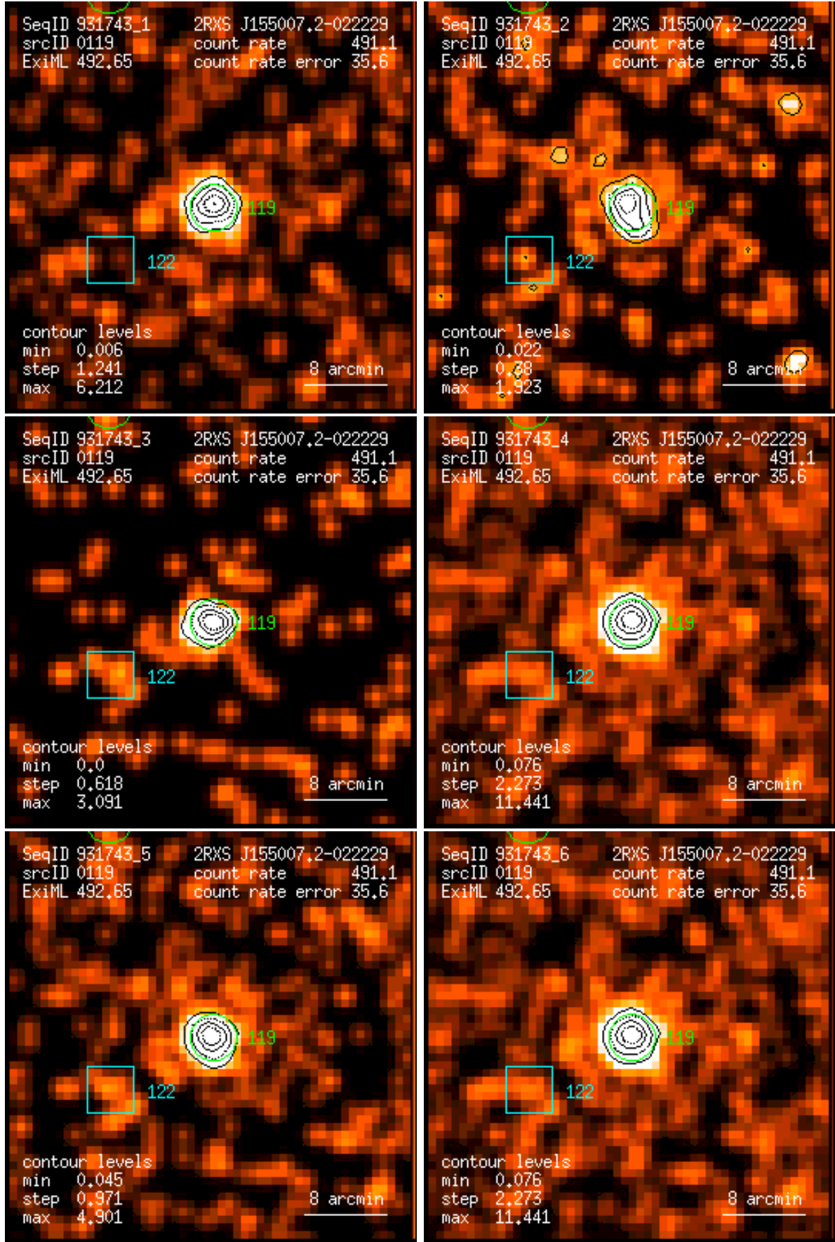
Figure 119: RASS 931743: detection 0119: band rate images, Gaussian filter: (1) PSPC channels 11 – 41, (2) 52 – 90, (3) 91 – 201, (4) 11 – 235, (5) 52 – 201, (6) 11 – 201. Broad band rates in counts/ks. Band rate contour levels in counts/ks/arcmin 2 .
