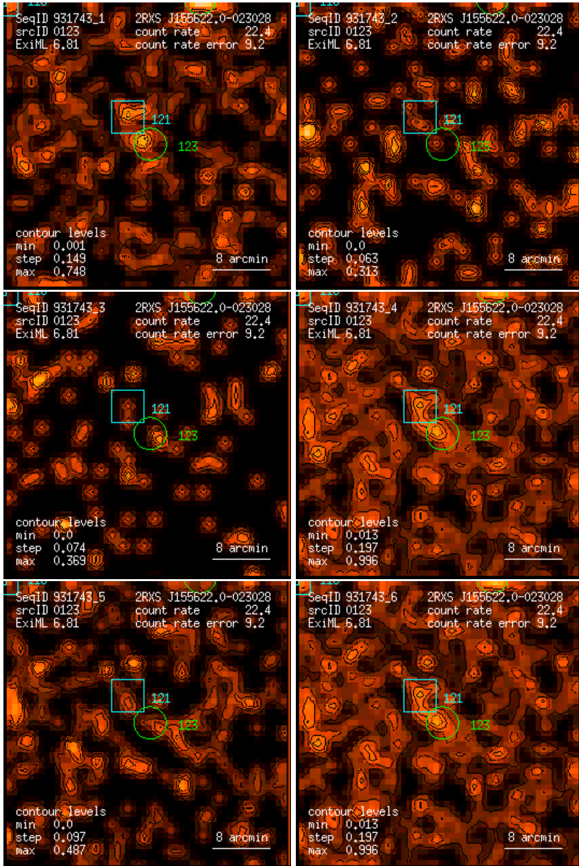
Figure 123: RASS 931743: detection 0123: band rate images, Gaussian filter: (1) PSPC channels 11 – 41, (2) 52 – 90, (3) 91 – 201, (4) 11 – 235, (5) 52 – 201, (6) 11 – 201. Broad band rates in counts/ks. Band rate contour levels in counts/ks/arcmin 2 .
