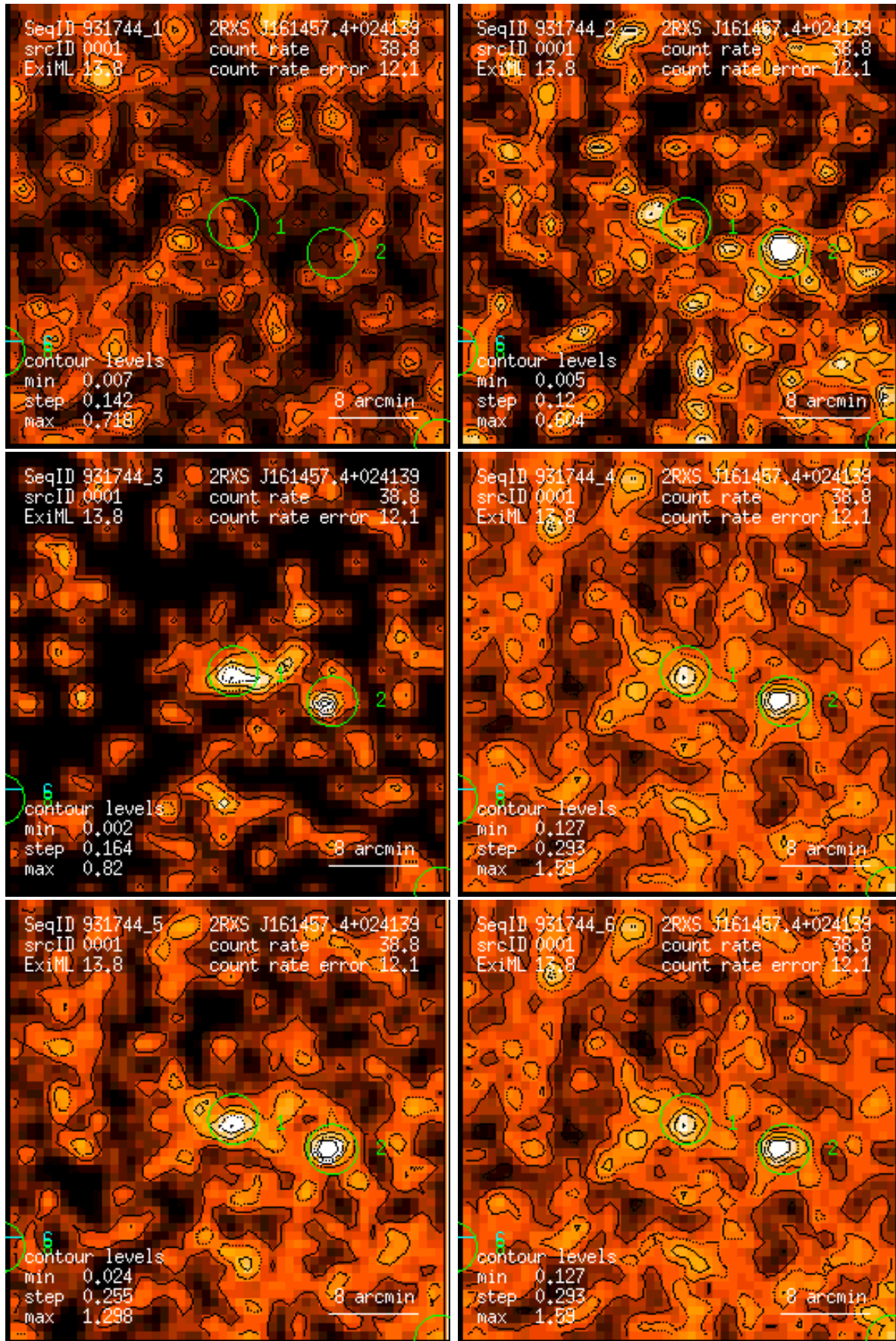
Figure 1: RASS 931744: detection 0001: band rate images, Gaussian filter: (1) PSPC channels 11 – 41, (2) 52 – 90, (3) 91 – 201, (4) 11 – 235, (5) 52 – 201, (6) 11 – 201. Broad band rates in counts/ks. Band rate contour levels in counts/ks/arcmin 2 .
