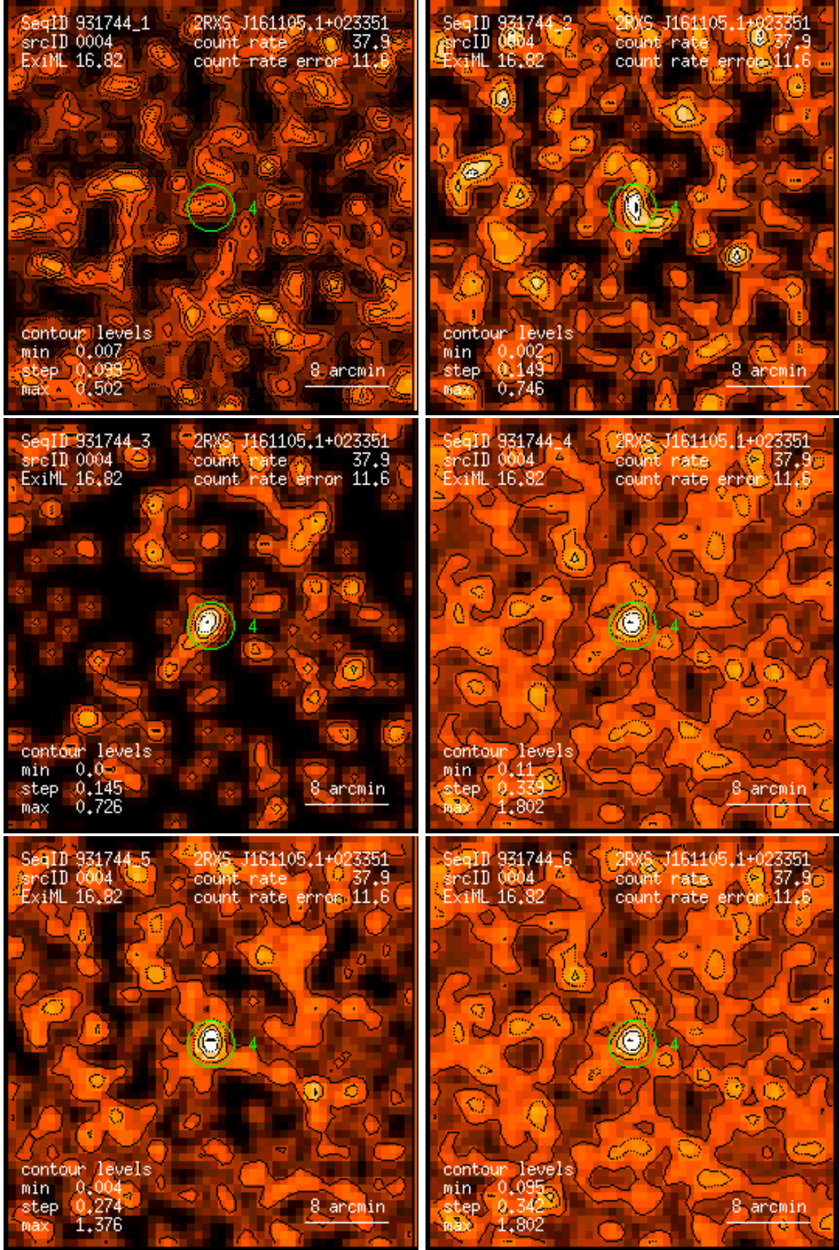
Figure 4: RASS 931744: detection 0004: band rate images, Gaussian filter: (1) PSPC channels 11 – 41, (2) 52 – 90, (3) 91 – 201, (4) 11 – 235, (5) 52 – 201, (6) 11 – 201. Broad band rates in counts/ks. Band rate contour levels in counts/ks/arcmin 2 .
