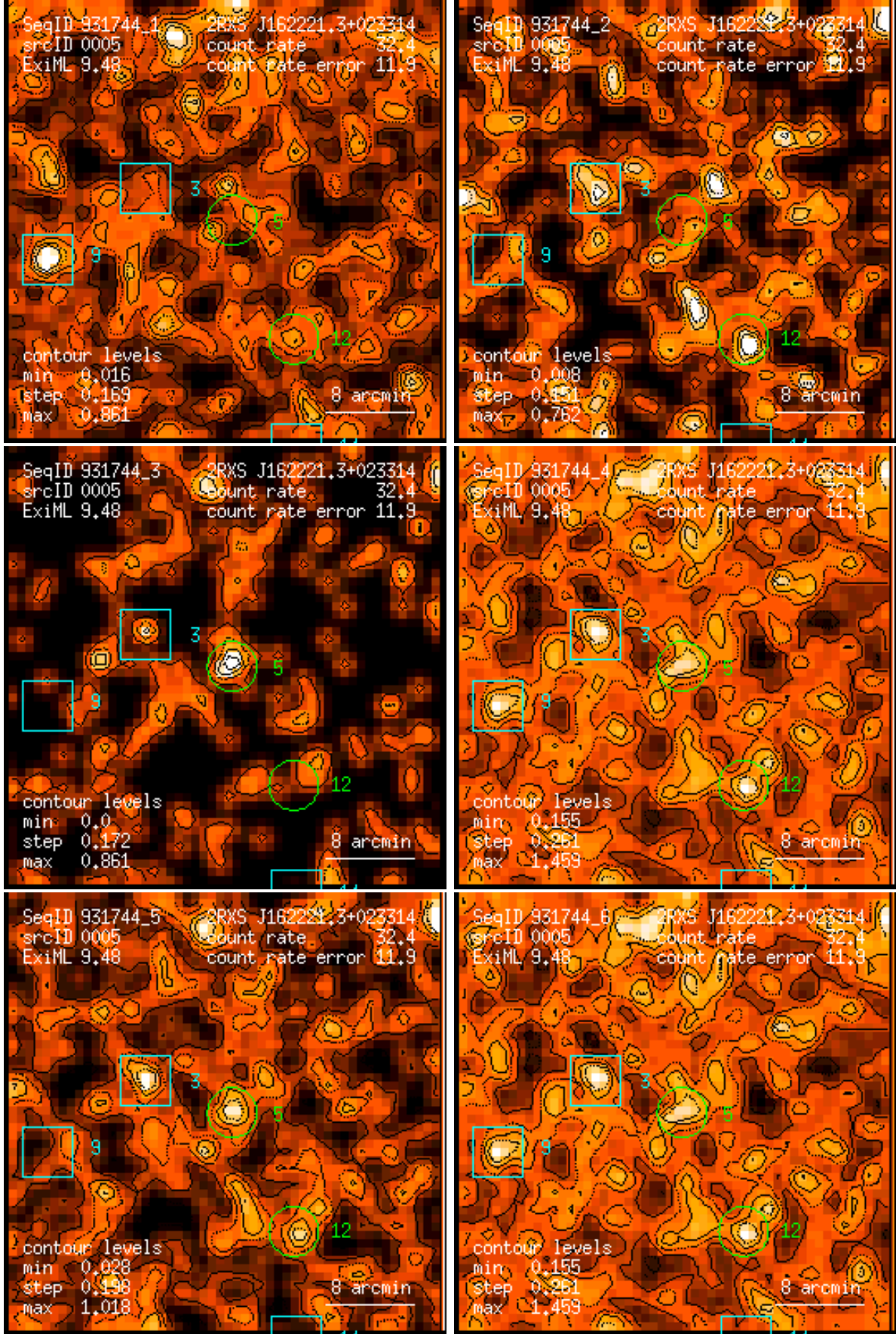
Figure 5: RASS 931744: detection 0005: band rate images, Gaussian filter: (1) PSPC channels 11 – 41, (2) 52 – 90, (3) 91 – 201, (4) 11 – 235, (5) 52 – 201, (6) 11 – 201. Broad band rates in counts/ks. Band rate contour levels in counts/ks/arcmin 2 .
