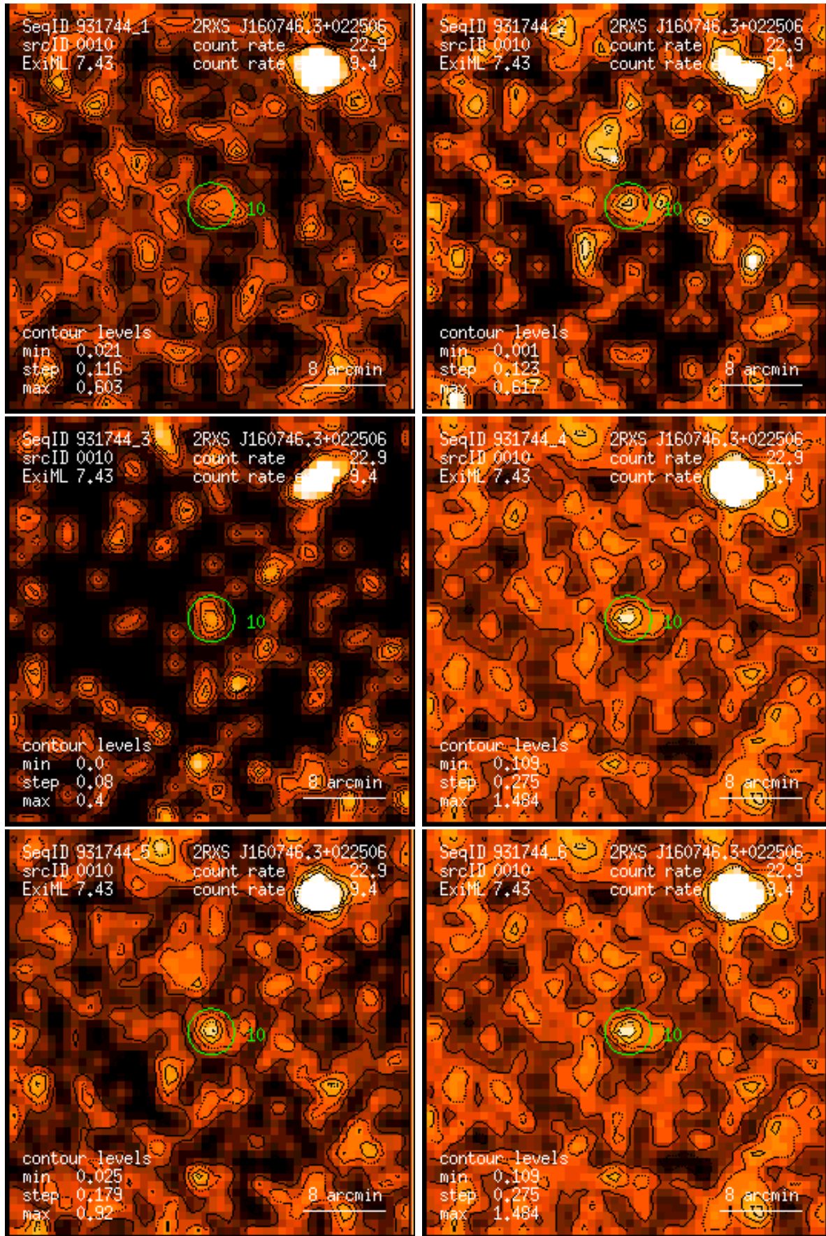
Figure 10: RASS 931744: detection 0010: band rate images, Gaussian filter: (1) PSPC channels 11 – 41, (2) 52 – 90, (3) 91 – 201, (4) 11 – 235, (5) 52 – 201, (6) 11 – 201. Broad band rates in counts/ks. Band rate contour levels in counts/ks/arcmin 2 .
