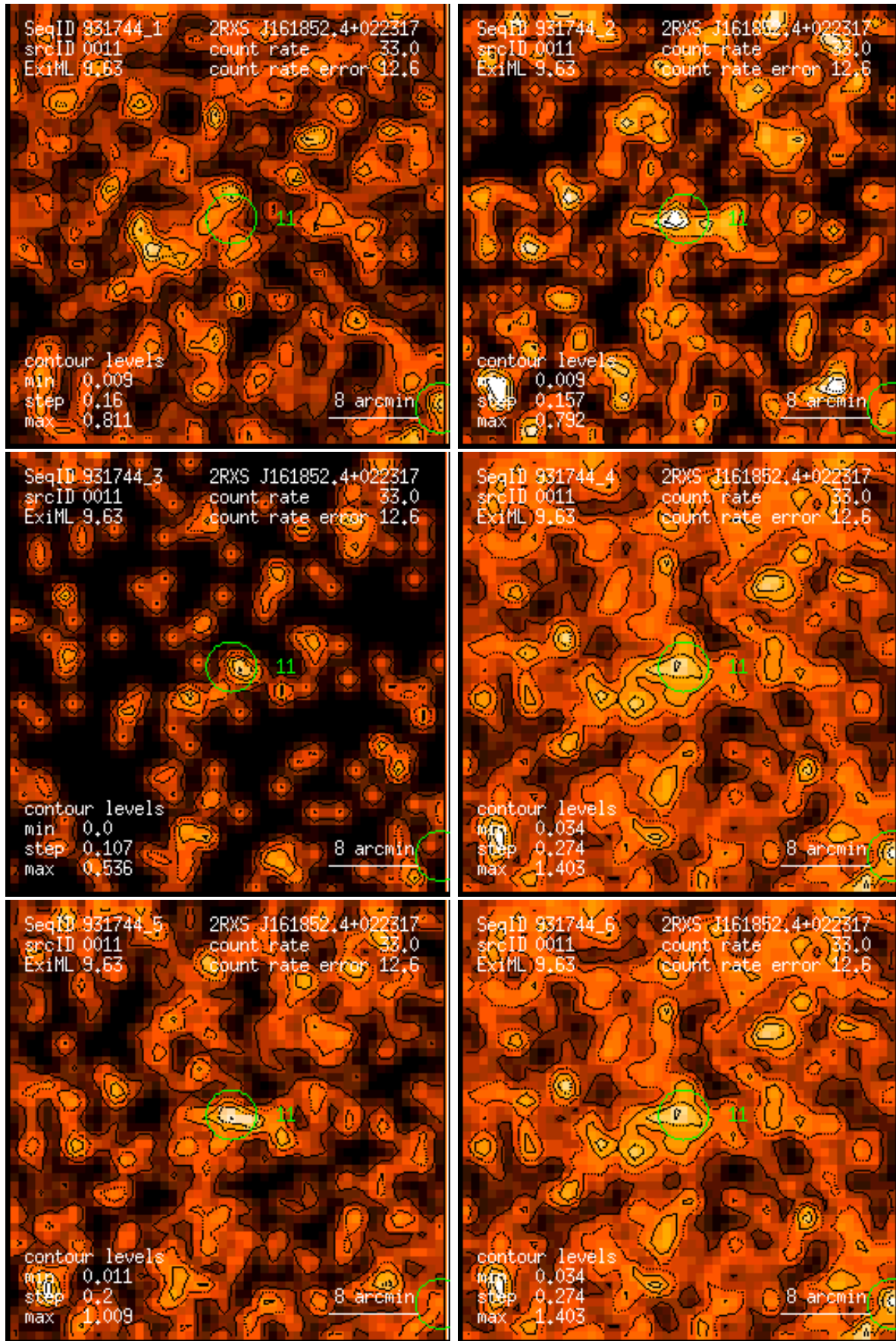
Figure 11: RASS 931744: detection 0011: band rate images, Gaussian filter: (1) PSPC channels 11 – 41, (2) 52 – 90, (3) 91 – 201, (4) 11 – 235, (5) 52 – 201, (6) 11 – 201. Broad band rates in counts/ks. Band rate contour levels in counts/ks/arcmin 2 .
