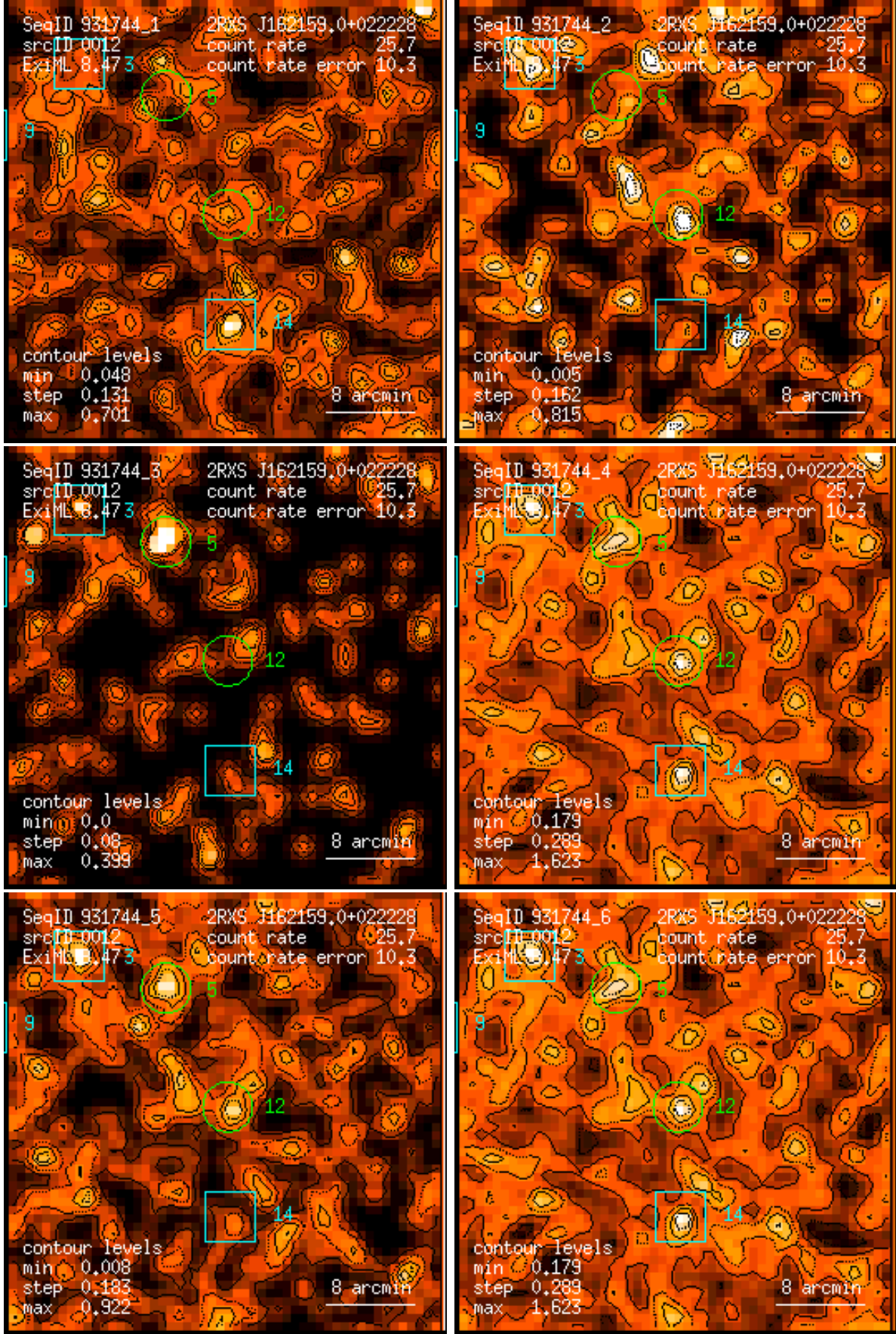
Figure 12: RASS 931744: detection 0012: band rate images, Gaussian filter: (1) PSPC channels 11 – 41, (2) 52 – 90, (3) 91 – 201, (4) 11 – 235, (5) 52 – 201, (6) 11 – 201. Broad band rates in counts/ks. Band rate contour levels in counts/ks/arcmin 2 .
