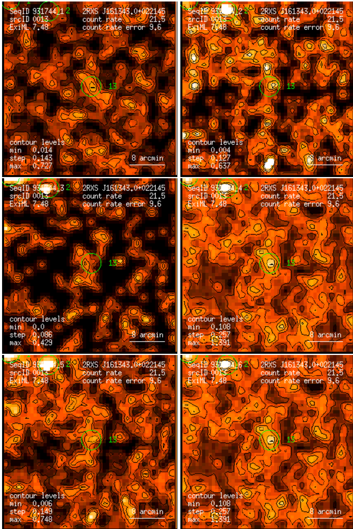
Figure 13: RASS 931744: detection 0013: band rate images, Gaussian filter: (1) PSPC channels 11 – 41, (2) 52 – 90, (3) 91 – 201, (4) 11 – 235, (5) 52 – 201, (6) 11 – 201. Broad band rates in counts/ks. Band rate contour levels in counts/ks/arcmin 2 .
