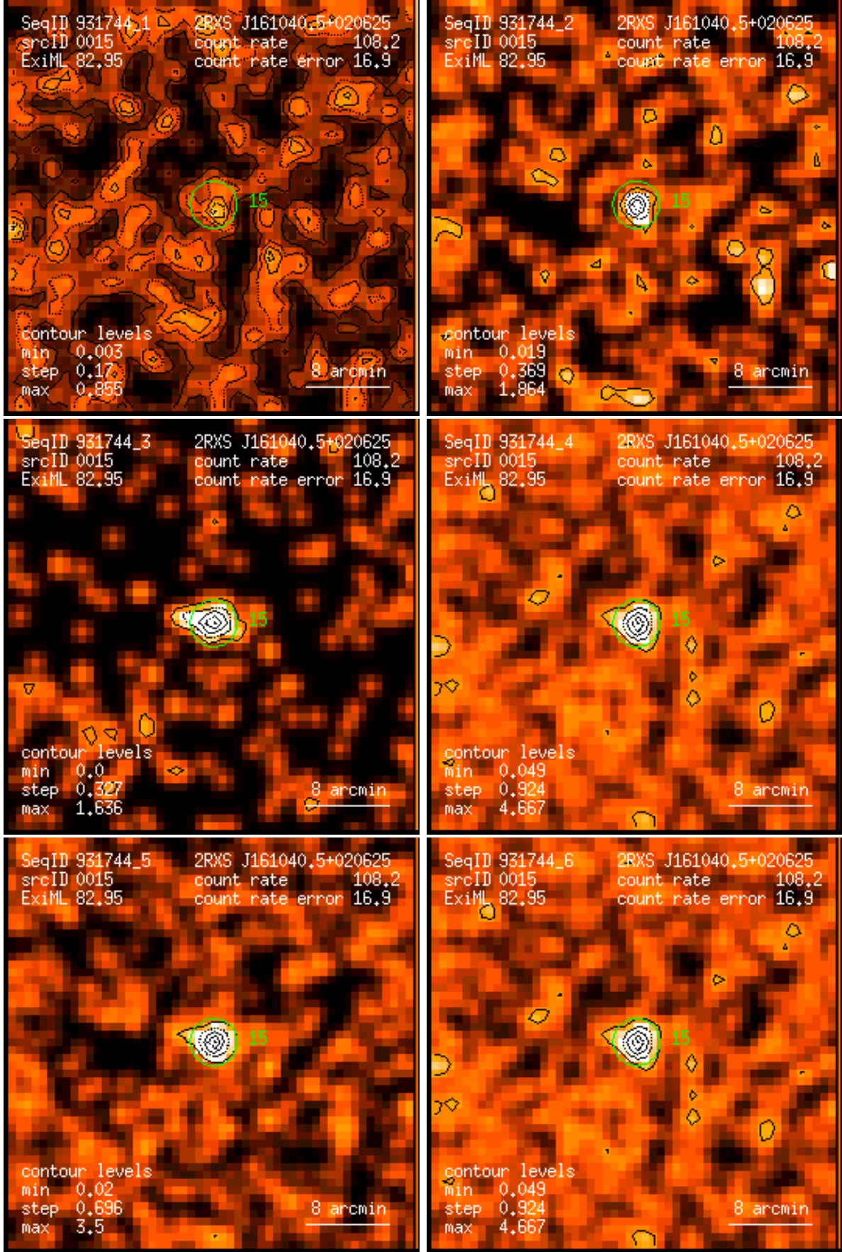
Figure 15: RASS 931744: detection 0015: band rate images, Gaussian filter: (1) PSPC channels 11 – 41, (2) 52 – 90, (3) 91 – 201, (4) 11 – 235, (5) 52 – 201, (6) 11 – 201. Broad band rates in counts/ks. Band rate contour levels in counts/ks/arcmin 2 .
