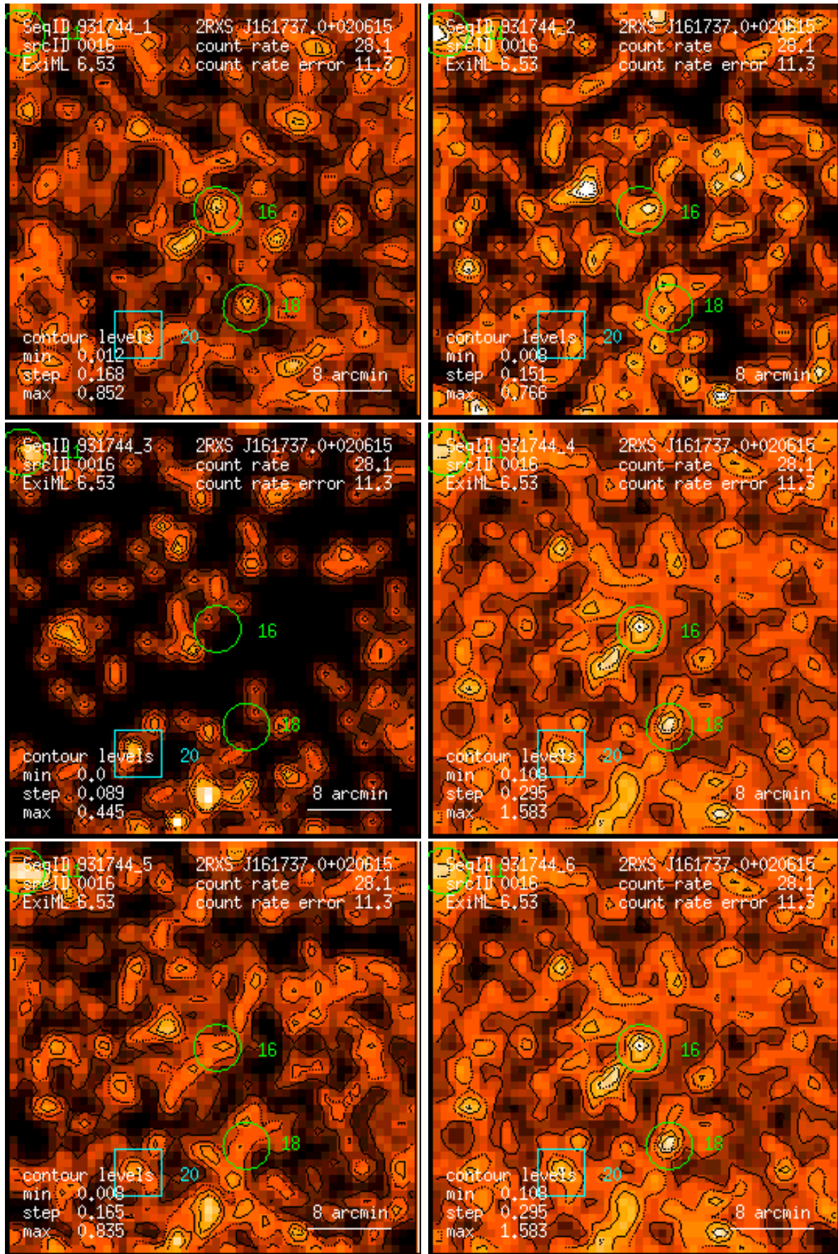
Figure 16: RASS 931744: detection 0016: band rate images, Gaussian filter: (1) PSPC channels 11 – 41, (2) 52 – 90, (3) 91 – 201, (4) 11 – 235, (5) 52 – 201, (6) 11 – 201. Broad band rates in counts/ks. Band rate contour levels in counts/ks/arcmin 2 .
