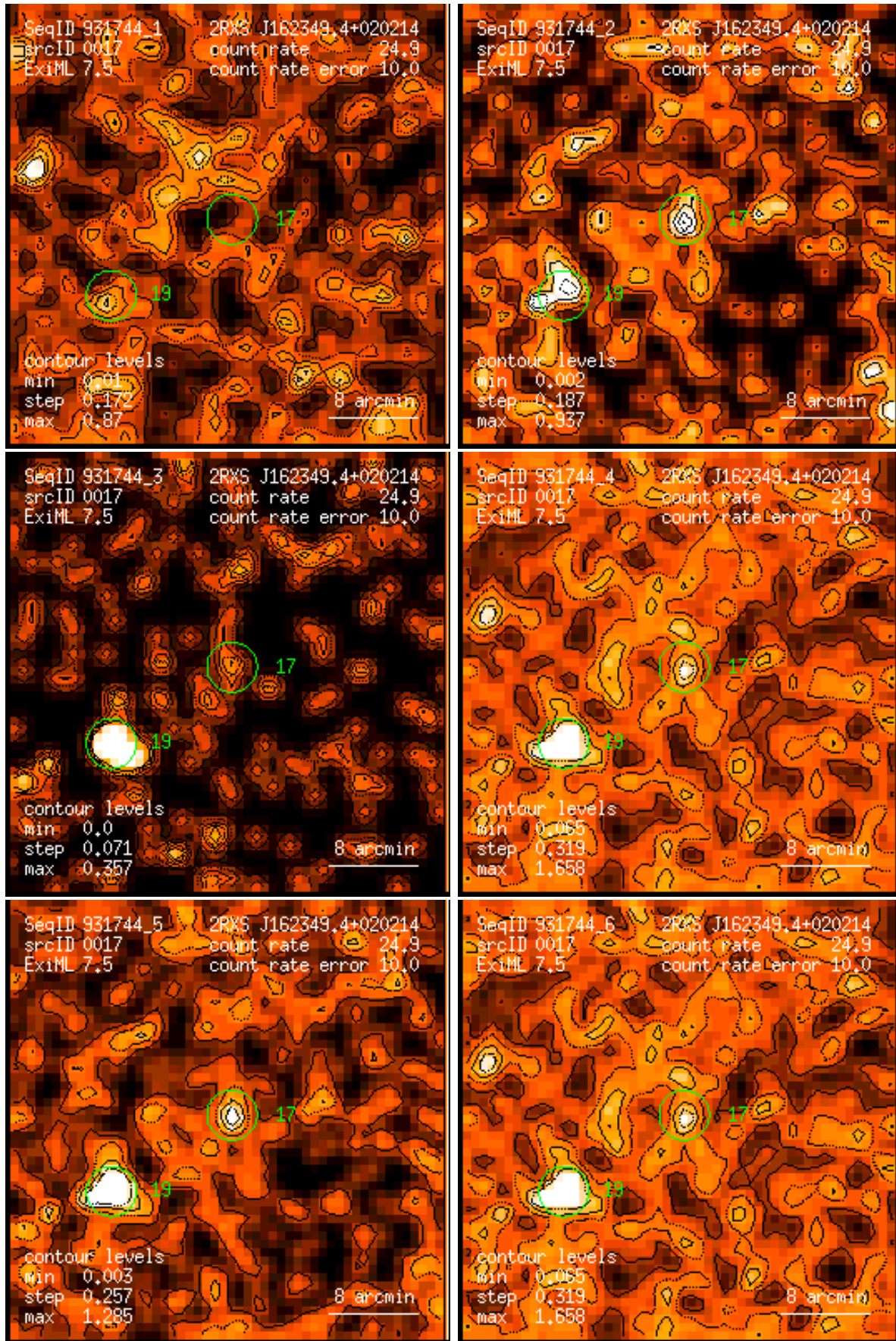
Figure 17: RASS 931744: detection 0017: band rate images, Gaussian filter: (1) PSPC channels 11 – 41, (2) 52 – 90, (3) 91 – 201, (4) 11 – 235, (5) 52 – 201, (6) 11 – 201. Broad band rates in counts/ks. Band rate contour levels in counts/ks/arcmin 2 .
