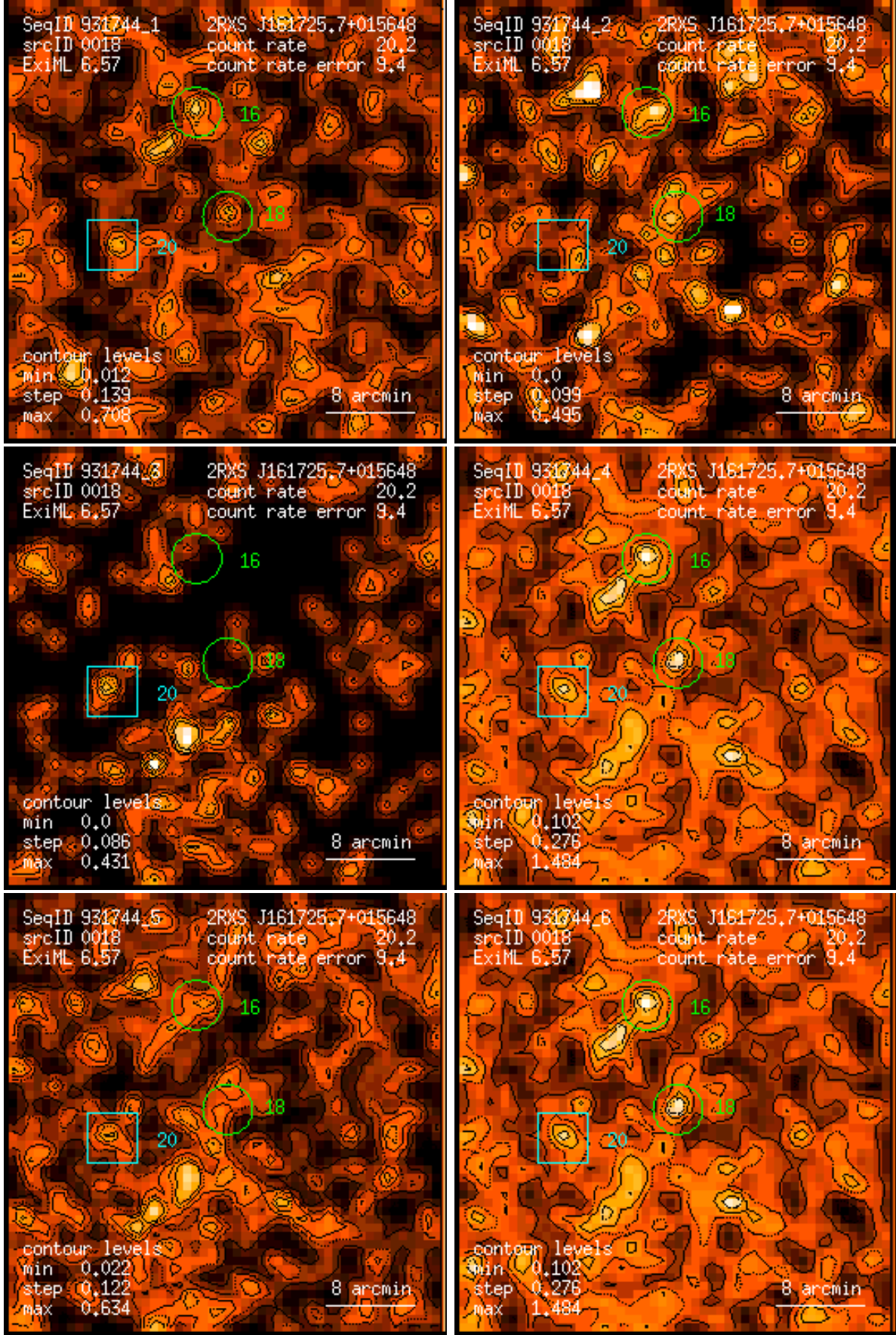
Figure 18: RASS 931744: detection 0018: band rate images, Gaussian filter: (1) PSPC channels 11 – 41, (2) 52 – 90, (3) 91 – 201, (4) 11 – 235, (5) 52 – 201, (6) 11 – 201. Broad band rates in counts/ks. Band rate contour levels in counts/ks/arcmin 2 .
